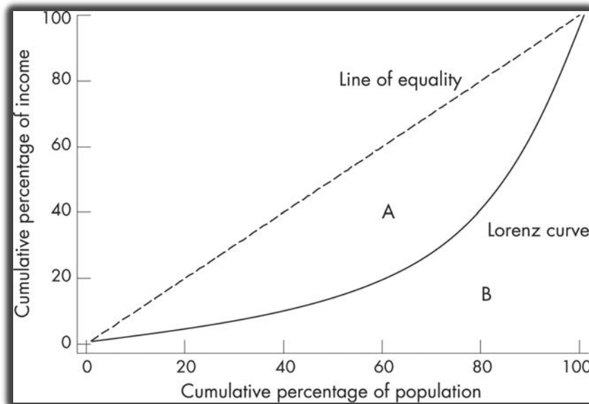
Figure 2. Lorenz Curve 24
