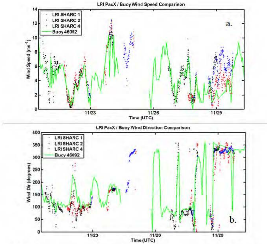
Figure 37. Same as Figure 35, except for a) wind speed; b) wind direction measurements.
