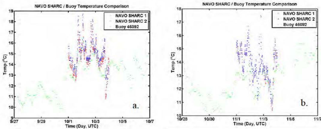
Figure 47. Same as Figure 45, except for air temperature.
