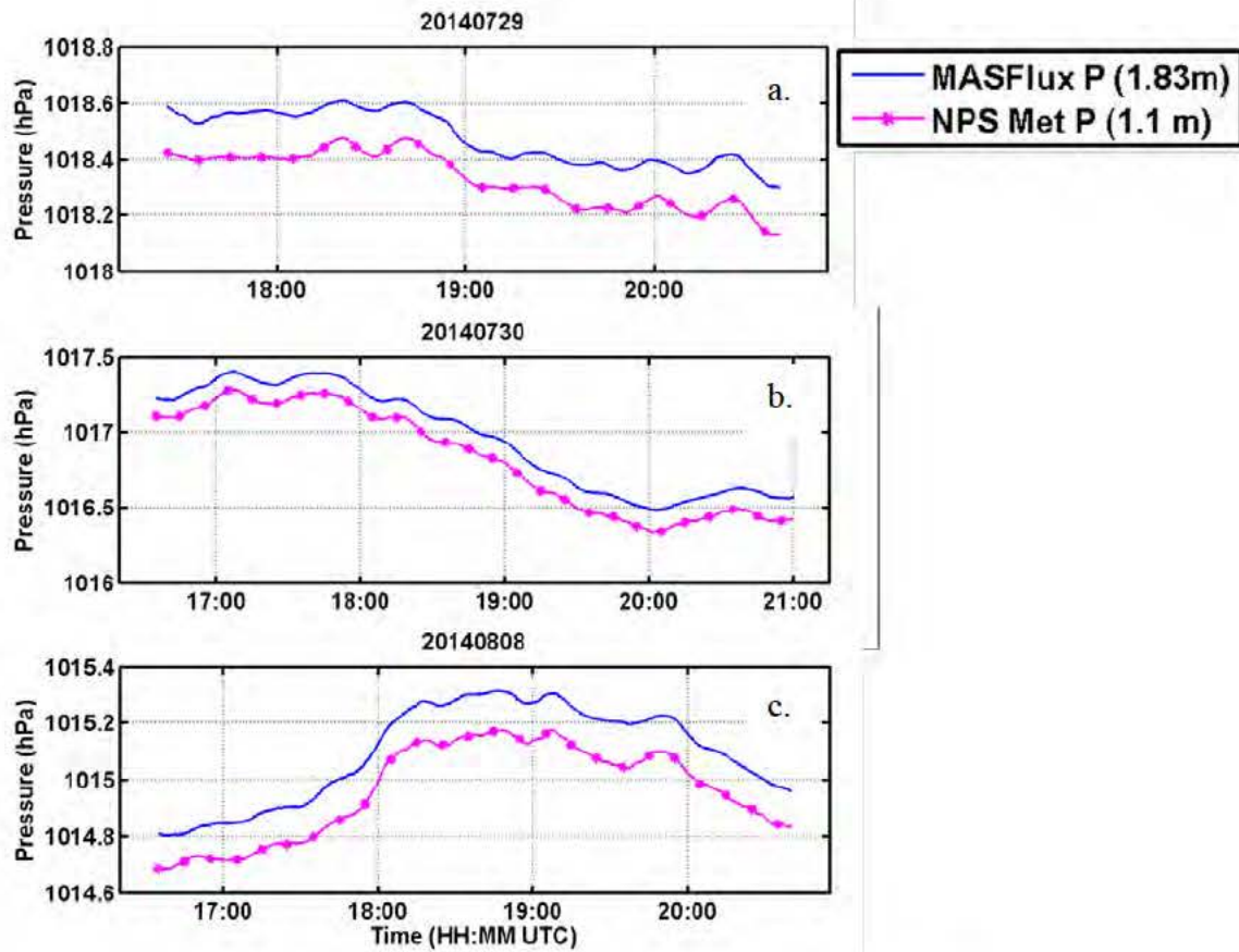
Figure 21. Same as Figure 15, except for pressure.
