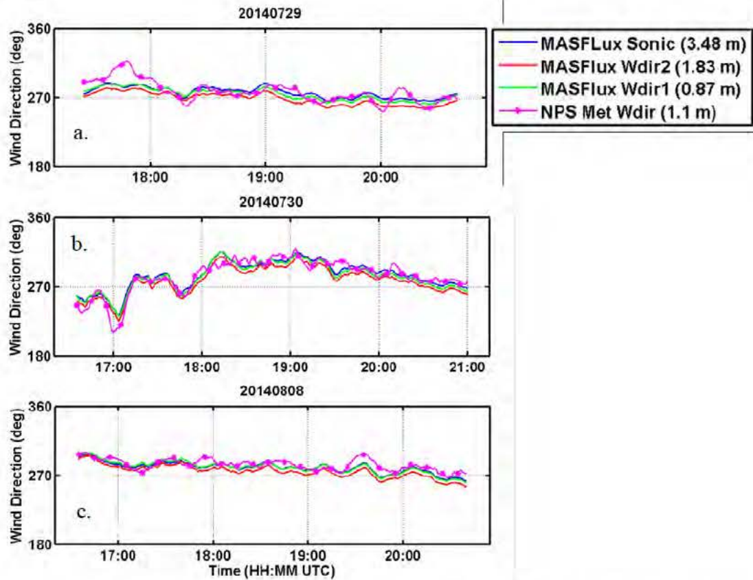
Figure 17. Same as Figure 15, except for wind direction.
