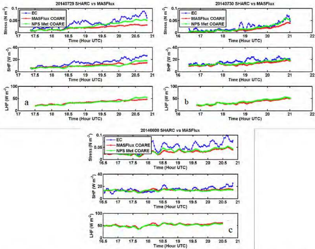
Figure 49. Time variation of NPS Met and MASFlux surface fluxes derived using mean measurements and COARE, and the fluxes from the EC method on a) July 29, 2014; b) July 30, 2014; c) August 8, 2014.
