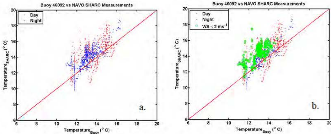
Figure 48. Same as Figure 41, except for the NAVO SHARC.
