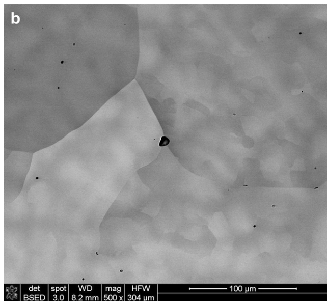
Fig. 2. SEM backscatter electron images of a polished cross-section of W–Nb–Mo–Ta alloy taken at two different magnifications.
