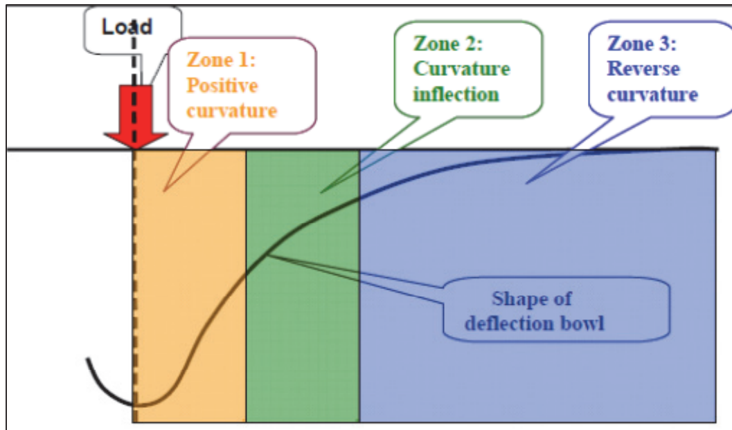
Figure 16. Curvature zones of a deflection basin (bowl) (from Horak and Emery 2009).
