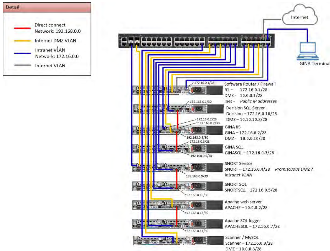
Figure 12. Conceptualized Hardware Configuration for RAMPART. The system was comprised of 9 servers separated into 3 VLANs to segregate network traffic. The red lines indicate the direct connection between databases.
