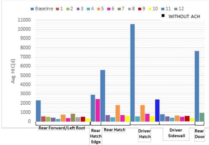
Figure 8: Vehicle B HIC(d)
