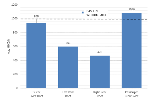
Figure 14: Vehicle A Roof Position Head Impact Testing
