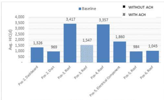
Figure 22: Vehicle C Baseline HIC(d)
