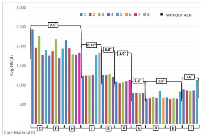
Figure 11: AoA Flat Fixture Material Thickness
