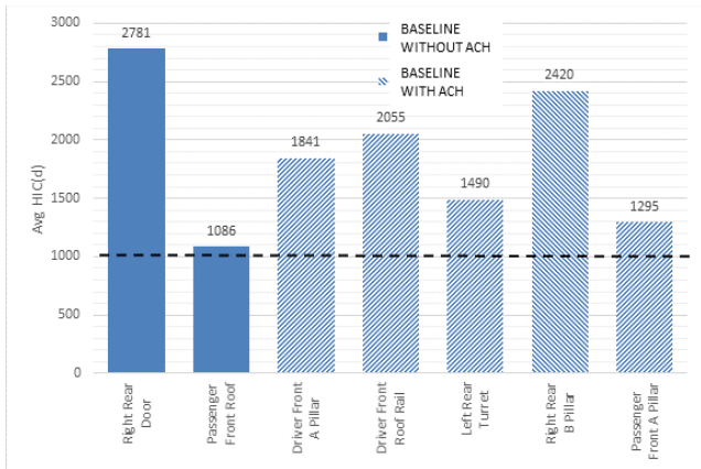
Figure 13: Vehicle A Positions that Exceeds Threshold
