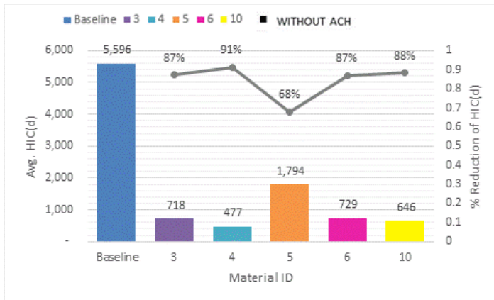
Figure 18: Rear Hatch HIC(d) and Percent Reduction
