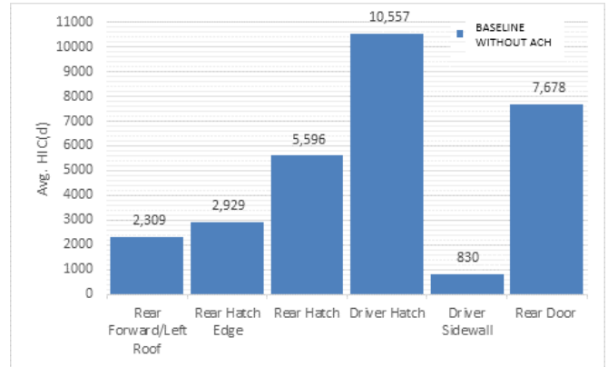
Figure 15: Vehicle B Baseline Head Impact Testing
