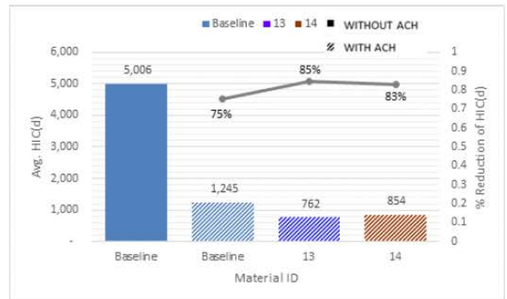
Figure 24: Roof HIC(d) and Percent Reduction
