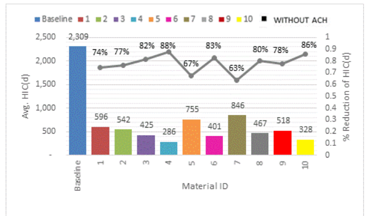
Figure 16: Rear Forward/Left Roof HIC(d) and Percent Reduction
