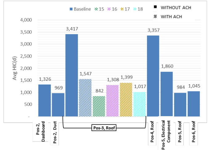
Figure 9: Vehicle C HIC(d)
