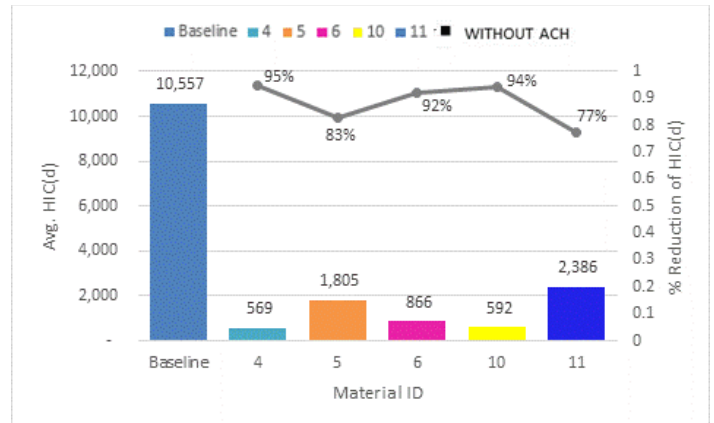
Figure 19: Driver Hatch HIC(d) and Percent Reduction
