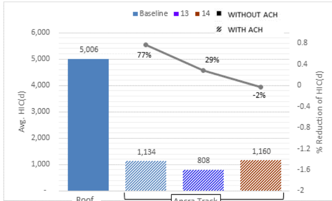
Figure 25: Ancra Track HIC(d) and Percent Reduction
