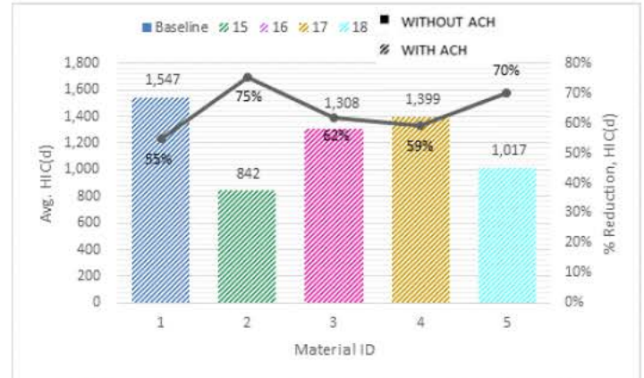
Figure 23: Pos-3 Avg. HIC(d) and Percent Reduction
