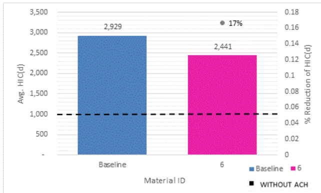
Figure 17: Rear Hatch Edge HIC(d) and Percent Reduction
