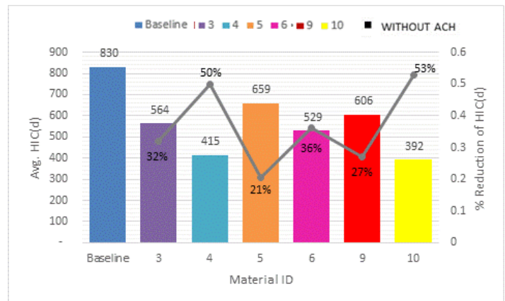
Figure 20: Driver Sidewall HIC(d) and Percent Reduction
