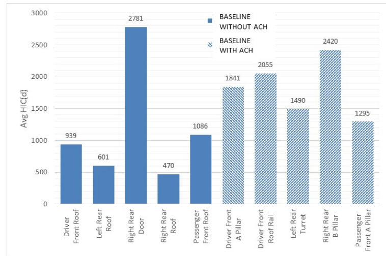
Figure 7: Vehicle A HIC(d)
