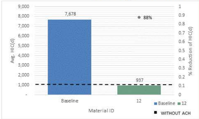
Figure 21: Rear Door HIC(d) and Percent Reduction
