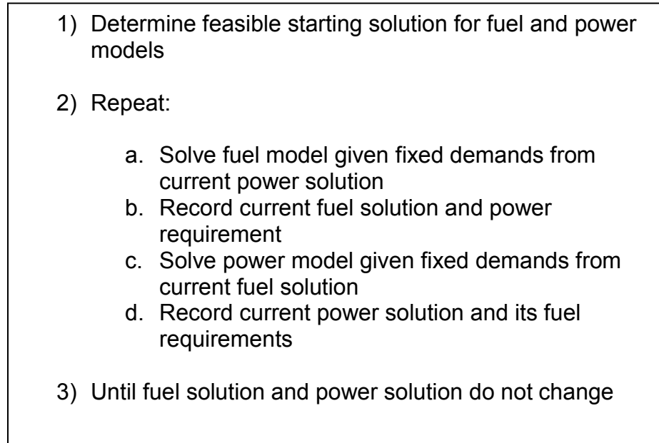
Figure 10. Pseudocode of iterative algorithm to solve for interdependent operation of fuel and electric power systems.
