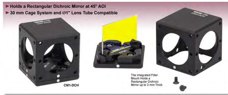
Figure 19. Catalog image of a CM1 series cage-cube from [36].
