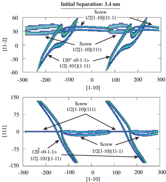
Figure 7. [111] ( x-y plane) and [11\bar{2}] ( x-z plane) projections of the partially cross slipped core structure for a screw 120^\circ intersection in fcc Ni from atomistic simulations when the initial separation distance between the screw and intersecting dislocations was kept at 3.4 nm. Atoms with energy greater than the energy at a stacking fault are plotted. The axes dimensions are in units of Å.
