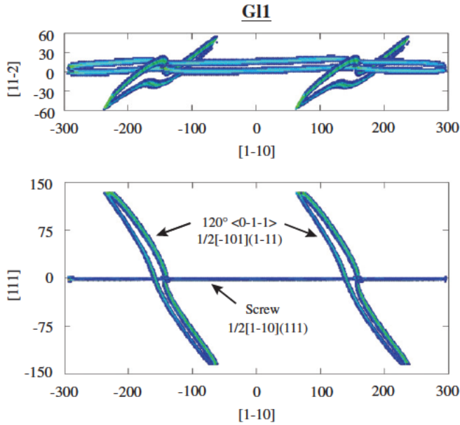
Figure 3. [111] ( x y plane) and [11\bar{2}] ( x z plane) projections of the core structure (G11) for a screw 120^\circ intersection in fcc Ni from atomistic simulations. Atoms with energy greater than the energy at a stacking fault are plotted. The axes dimensions are in units of Å.
