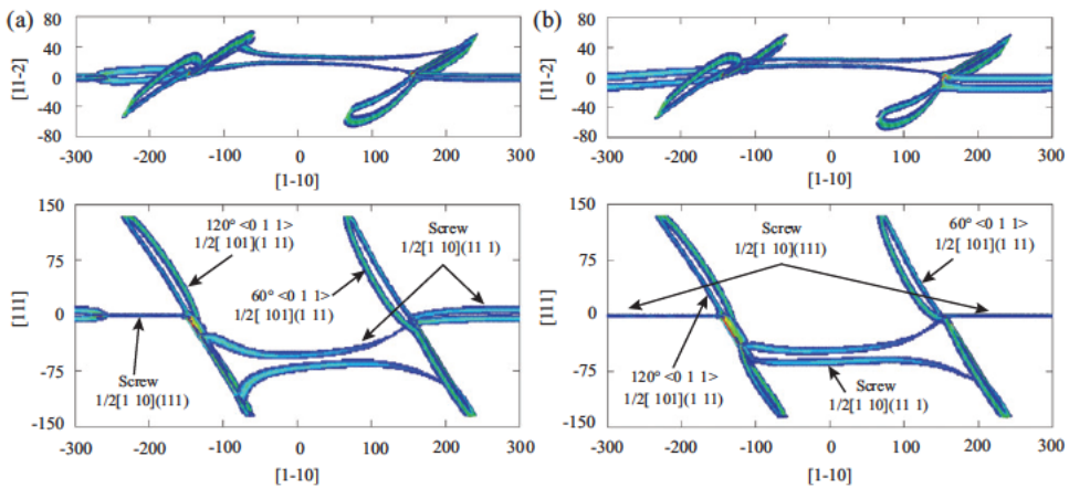
Figure 11. [11\bar{1}] ( x y plane) and [11\bar{2}] ( x z plane) projections of two different core structures obtained for screw 120^\circ and 60^\circ intersections in fcc Ni from atomistic simulations with periodic boundary conditions along the screw or 'x' direction. Atoms with energy greater than the energy at a stacking fault are plotted. The axes dimensions are in units of \text{\AA} .
