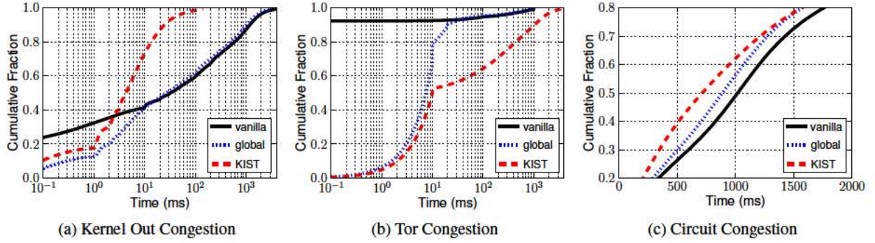
Figure 6: Congestion for vanilla Tor, KIST, and the global scheduling part of KIST (without enforcing write limits). Figures 6a and 6b show the distribution of cell congestion local to each relay (with logarithmic x-axes), while Figure 6c shows the distribution of the end-to-end circuit congestion for all measured cells.
