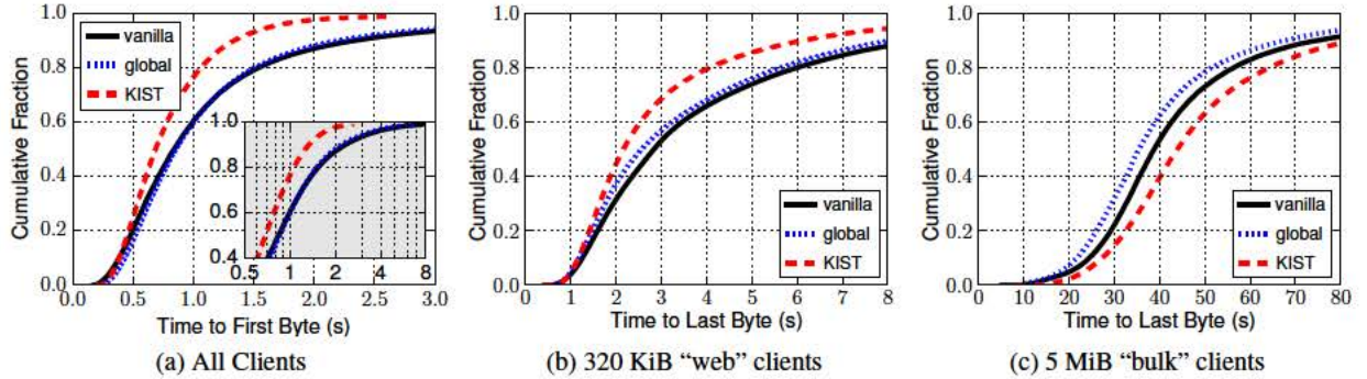
Figure 7: Client performance for vanilla Tor, KIST, and the global scheduling part of KIST (without enforcing write limits). Figure 7a shows the distribution of the time until the client receives the first byte of the data payload, for all clients, while the inset graph shows the same distribution with a logarithmic x-axis. Figures 7b and 7c show the distribution of time to complete a 320 KiB and 5 MiB file by the “web” and “bulk” clients, respectively.
