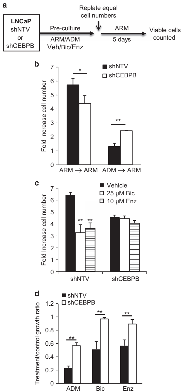
Figure 6. C/EBPβ is required for complete maintenance of growth arrest induced by AR inhibition in LNCaP cells. (a) LNCaP cells expressing shCEBPB or shNTV were pre-cultured in doxycycline under the indicated conditions or in ARM control media, 1.5E5 cells from each pre-culture condition were replated and enumerated after 5 days, as depicted in the diagram. (b) After 7 days pre-culture in ARM or ADM, equal number of shCEBPB or shNTV LNCaP cells were re-plated in ARM in a 6-well dish and counted 5 days later. The average fold increase in cell number is shown. (c) Similarly, cells were pre-cultured for 4 days with bicalutamide (Bic), enzalutamide (Enz) or vehicle control and doxycycline, re-plated in ARM and enumerated after 5 days as described above. (d) The relative growth ratio of cells pre-cultured in ADM, bicalutamide (Bic) or enzalutamide (Enz) over cells cultured in ARM control conditions. Bar graphs represent the mean of at least three experiments \pm s.e.m.; * P < 0.05 ; ** P < 0.005 .
