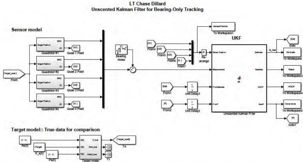
Figure 24. SIMULINK model for bearing-only tracking simulation, using an unscented Kalman filter and point-mass kinematics
