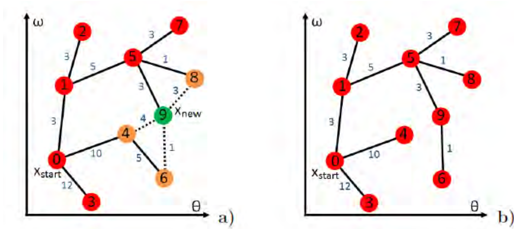
Figure 41. Visual display of RRT* rewiring step, from [28]
