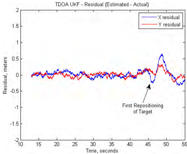
Figure 66. Continued convergence of estimated target location after first repositioning of helmet
