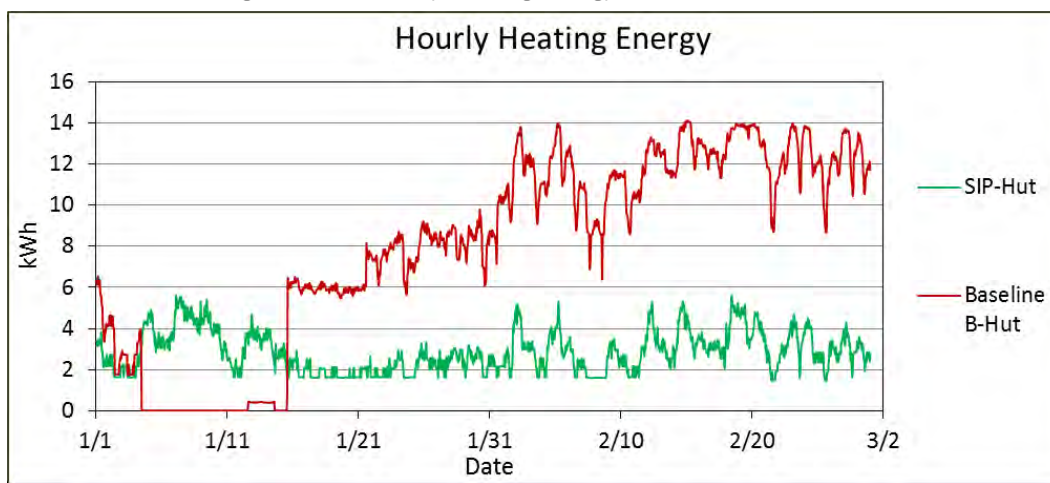
Figure 4-23. Hourly heating energy use in the test huts.
