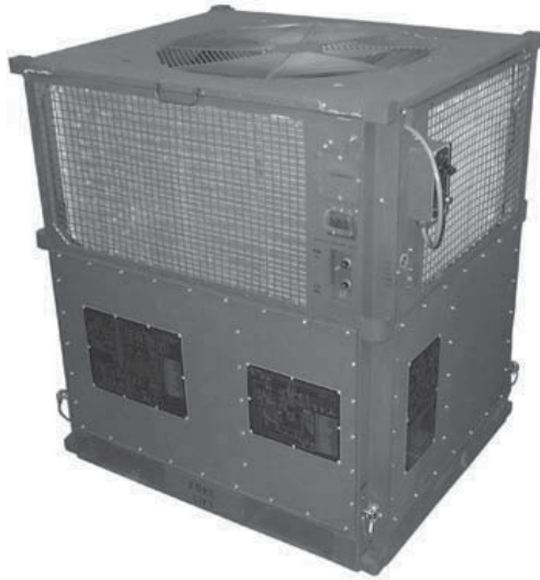
Figure 5-1. 60K Btu/hr IECU.
