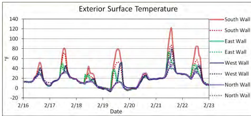
Figure 4-10. EnergyPlus calculated and measured exterior surface temperature before adjusting SR.
