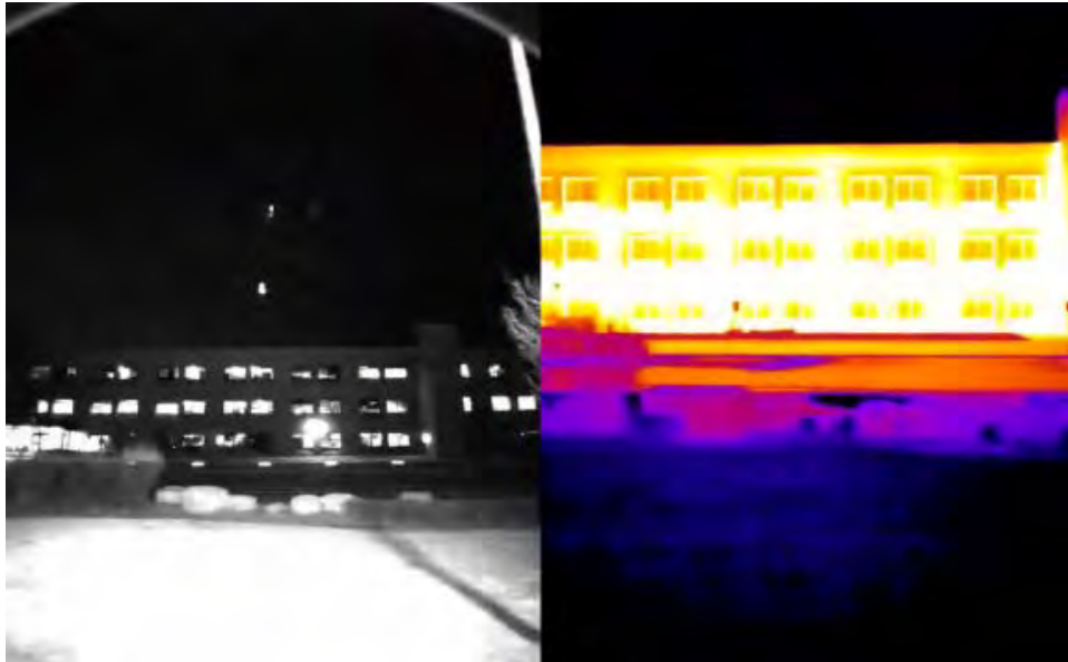
Figure D-86. NIR image (left) and thermal image (right) of Bldg 1600, Scott AFB.
