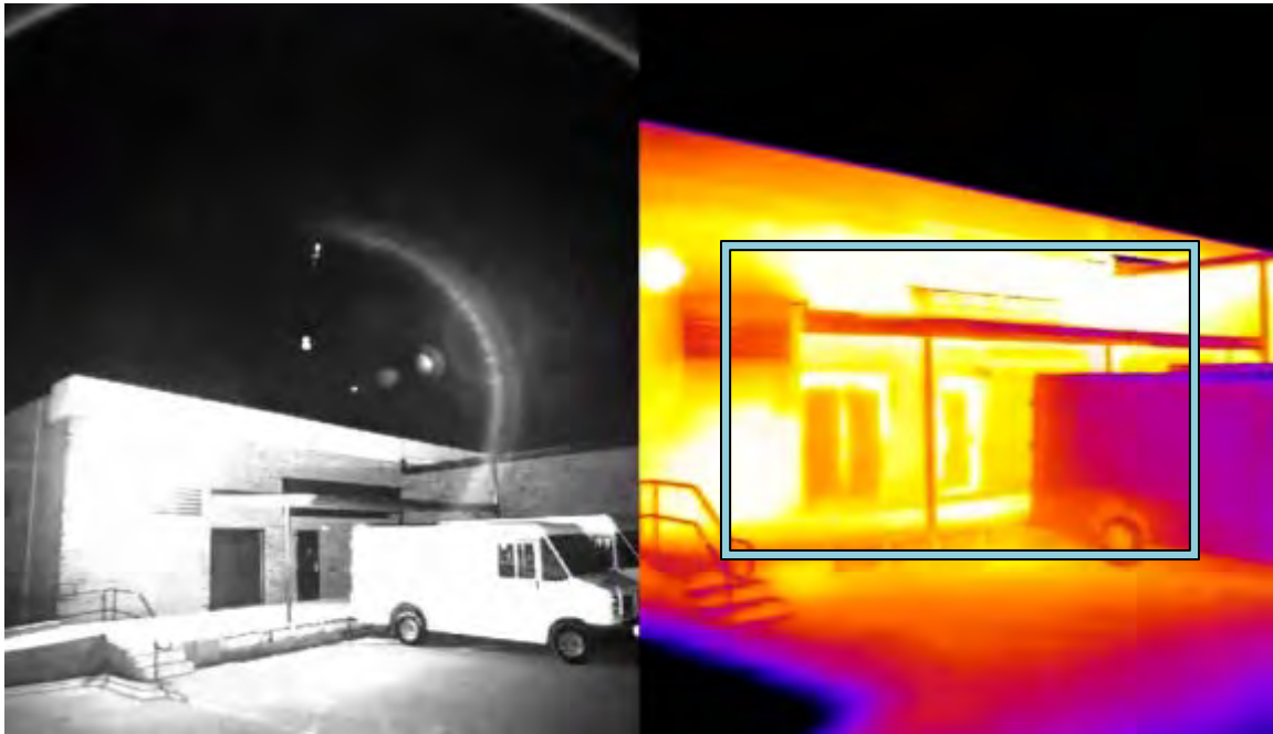
Figure D-90. NIR image (left) and thermal image (right) of Bldg 1650, Scott AFB.
