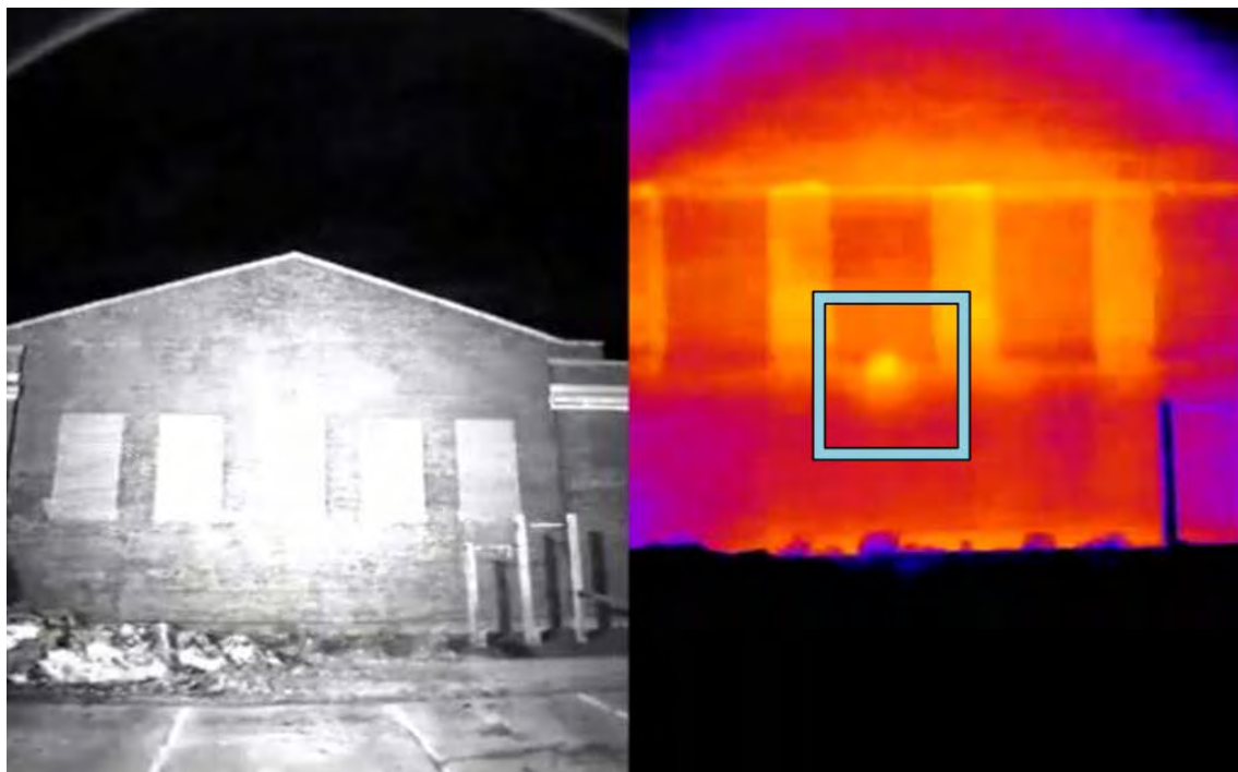
Figure D-8. NIR image (left) and thermal image (right) of Bldg 6, Scott AFB.
