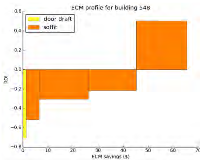
Figure D-48. ECM profile for Bldg 548, Scott AFB.
