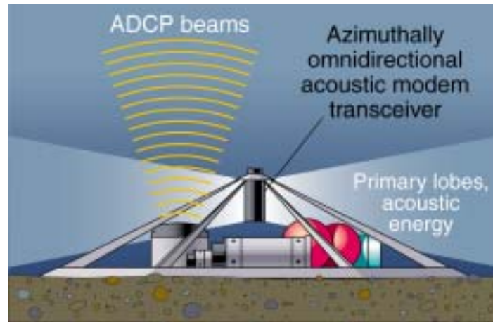
Figure 5. U Conn's ADCP sensor nodes are housed in seafloor frames having a low-profile pyramidal shape intended to deflect trawling gear. The telesonar modem 4-element vertical-line-array transducer resides in the apex of the frame and has a beampattern for azimuthally omnidirectional transmission and reception. All other components lie below the main lobe of the telesonar beampattern.
