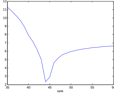
Figure 3.1: \left( \log \left( \text{LR}(\mathbf{R}_{\text{RCML}}(r), \mathbf{Z}) / \text{LR}_0 \right) \right)^2 versus r for KASSPER dataset ( K = 2N = 704 )
