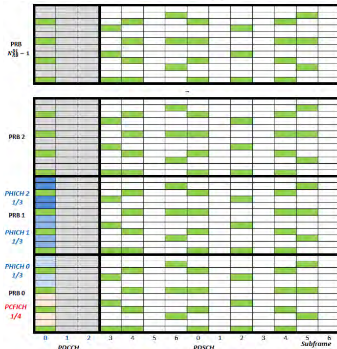
Figure 1: The time frequency resource plane for the downlink in the LTE standard. The grey region represents control information while the green regions reflect reference signals. The control signals occupy roughly a quarter of downlink transmission, and with the reference and measurement signals, the non-information bearing overhead in the downlink stands at about a third. LTE advanced required extra control and reference signals which further grew this fraction. See the tutorial for details and acronym definitions.
