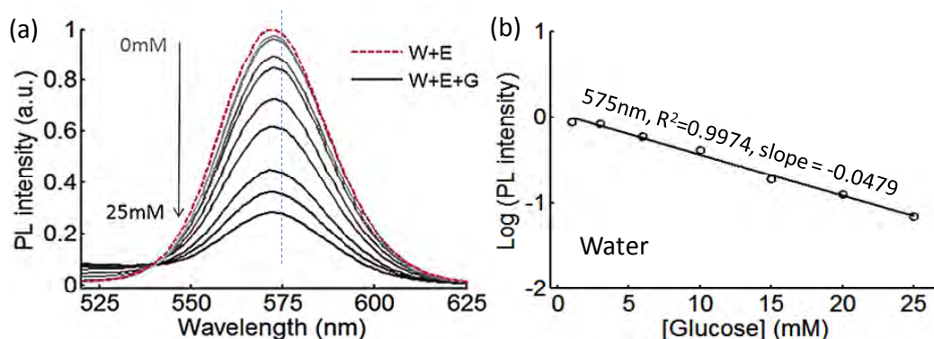
Figure 22. (a) Normalized 575-nm QD PL intensity curves for various concentrations of glucose (3.5μM, 4μM, 1mM, 3mM, 6mM, 10mM, 15mM, 20mM, 25mM). (b) Calibration curves for 575-nm QDs at a 1:100 dilution. The curve relate the measured PL intensity to the glucose concentration and are linear when plotted on a log-linear scale. All data is normalized to the PL intensity of a solution containing only water and enzymes (no glucose).
