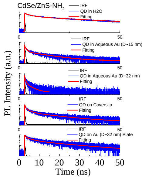
Figure 1. Fluorescence lifetime dynamics of NH 2 -functionalized CdSe/ZnS coreshells in water, on the surface of Au nanoparticles, and on the cover glass. The NH 2 functional group has a strong affinity with Au nanoparticles.
