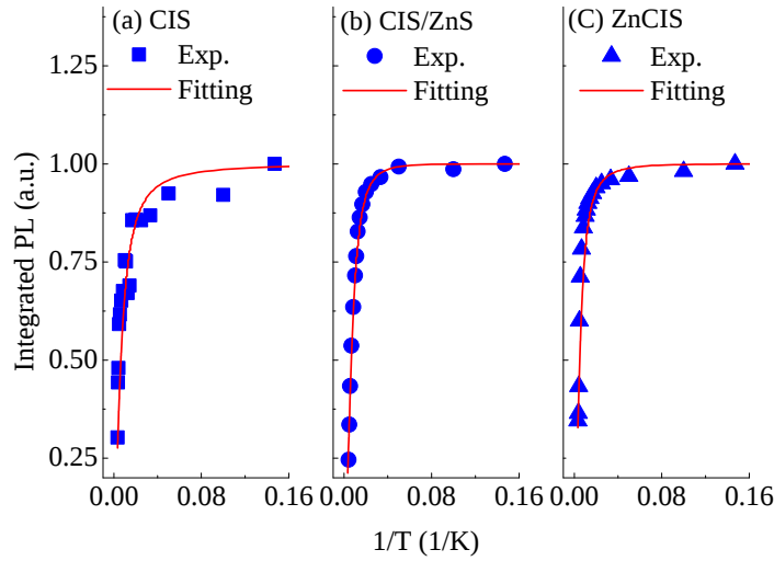
Figure 15. Thermal quenching properties of PLs from (a) CIS, (b) CIS/ZnS, and (c) ZnCIS.
