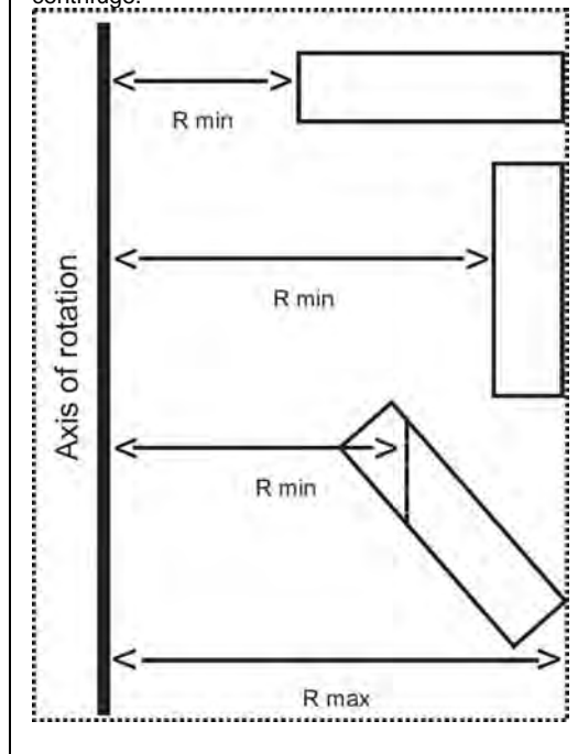
Figure 3. Determination of the minimum and maximum radius based on the geometry of a centrifuge.
