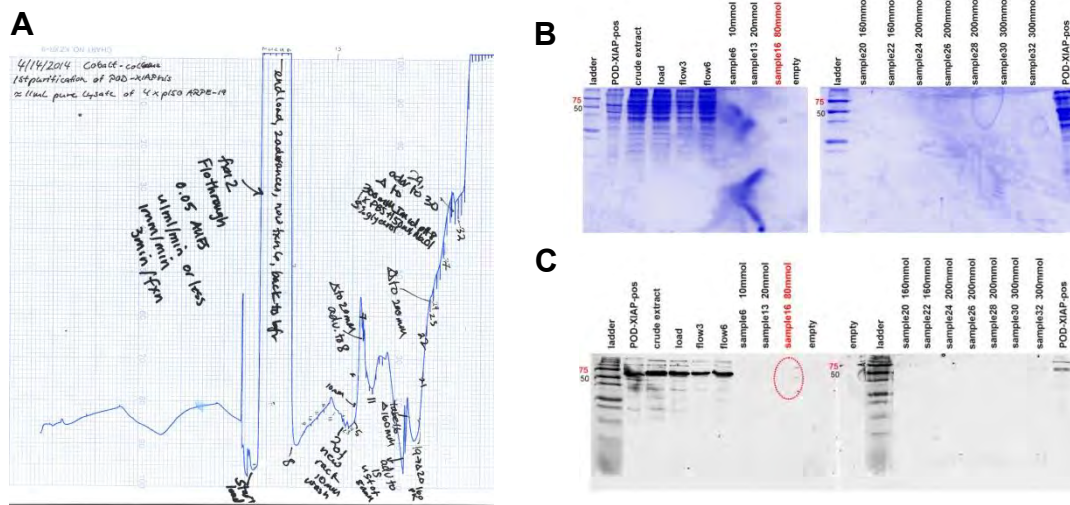
Figure 7: First Co 2+ -column purification of POD-XIAPhis
