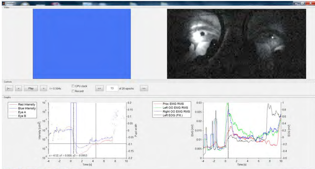
Figure 3. A screenshot of the Matlab GUI populated with example data from a human subject. The experiment setup consisted of a Diagnosys Ganzfeld bowl to present 1-second red and blue light stimuli, while an Arrington eye frame mounted eye tracker with miniature video cameras was used to collect pupil data, and a wired Biopac system collected EMG, EOG, etc. data. In this example, data are displayed for t=0.504s after stimulus onset (as indicated by the vertical black dotted line in each graph), at about the time when the EMG RMS and EOG values peak, as can be seen in the graph on the lower right hand side. Stimulus and pupillometry data are shown in the graph on the left hand side and in this case a one second blue stimulus was given (rectangular blue step in tracing). The left video frame shows that a blue stimulus is presented in the Diagnosys bowl at this time instance, and the right video frame shows the subject's face as seen from the built-in IR camera inside the bowl pointed at the subject. At this video frame, captured at the peak of the EMG response, it can be observed that the eyelids are partly squinted closed in response to the bright blue light stimulus, coinciding with the EMG tracing in the lower right graph.
