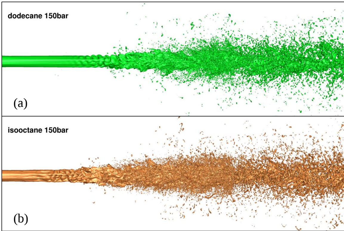
Figure 11. Detailed spray structure at isocontours of f=0.5 at t=100 us for (a) ndodecane and (b) isoctane at injection pressure of 150 bar.
