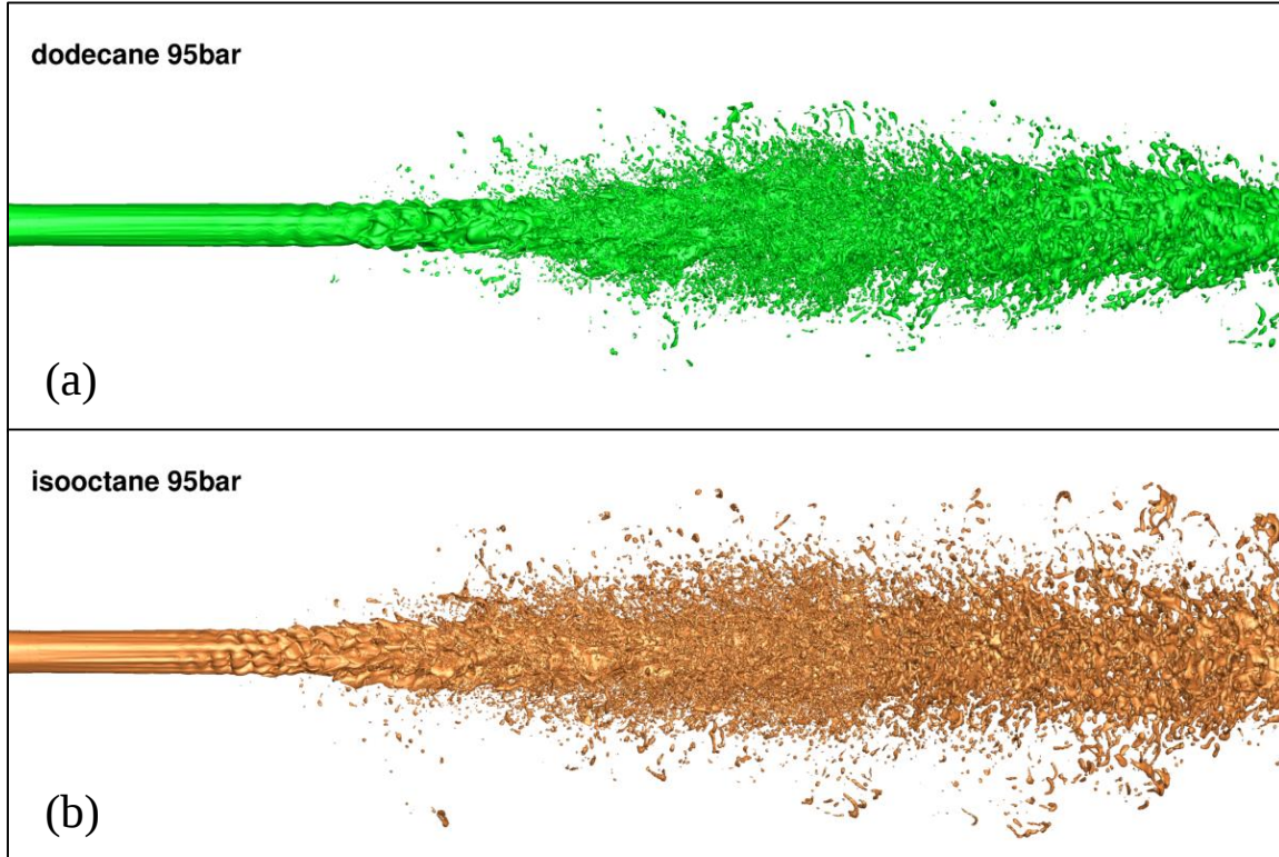
Figure 10. Detailed spray structure at isocontours of f=0.5 at t=100 us for (a) ndodecane and (b) isoctane at injection pressure of 95 bar.
