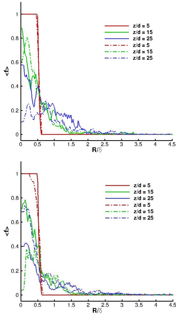
Figure 9. Radial distribution of mean VoF, \overline{f} , fields at t = 100 \mu s (0.1 ms) at three axial locations. Solid lines represent n-dodecane, dashed lines isoctane
