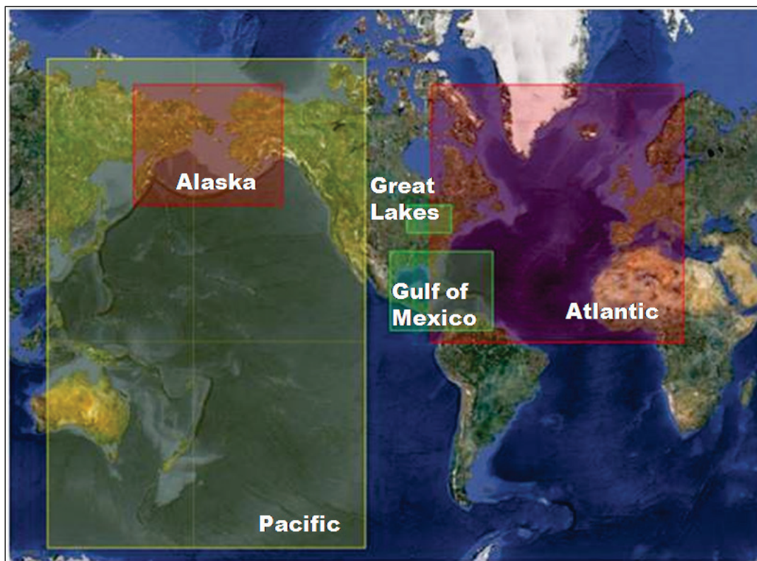
Figure 2. WIS wind and wave hindcast domains.
