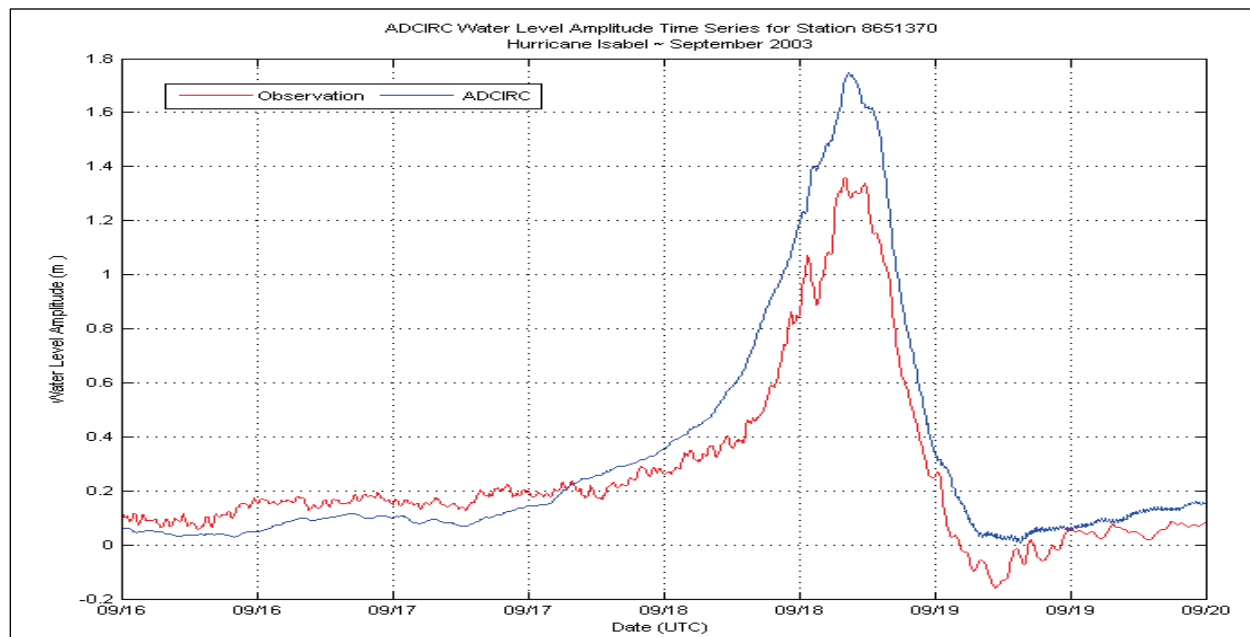
Figure 31. Comparison of FEMA RIII water level hindcast (blue) with observed water levels (red) during Hurricane Isabel (September 2003) at Duck.
