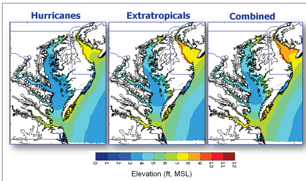
Figure 27. FEMA RIII 100 yr water levels (MSL) for hurricanes, extratropical storms, and all events (synthesis). Note: Water elevations are in feet.
