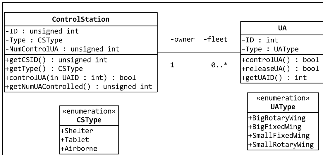
Figure 2. Class Diagram
