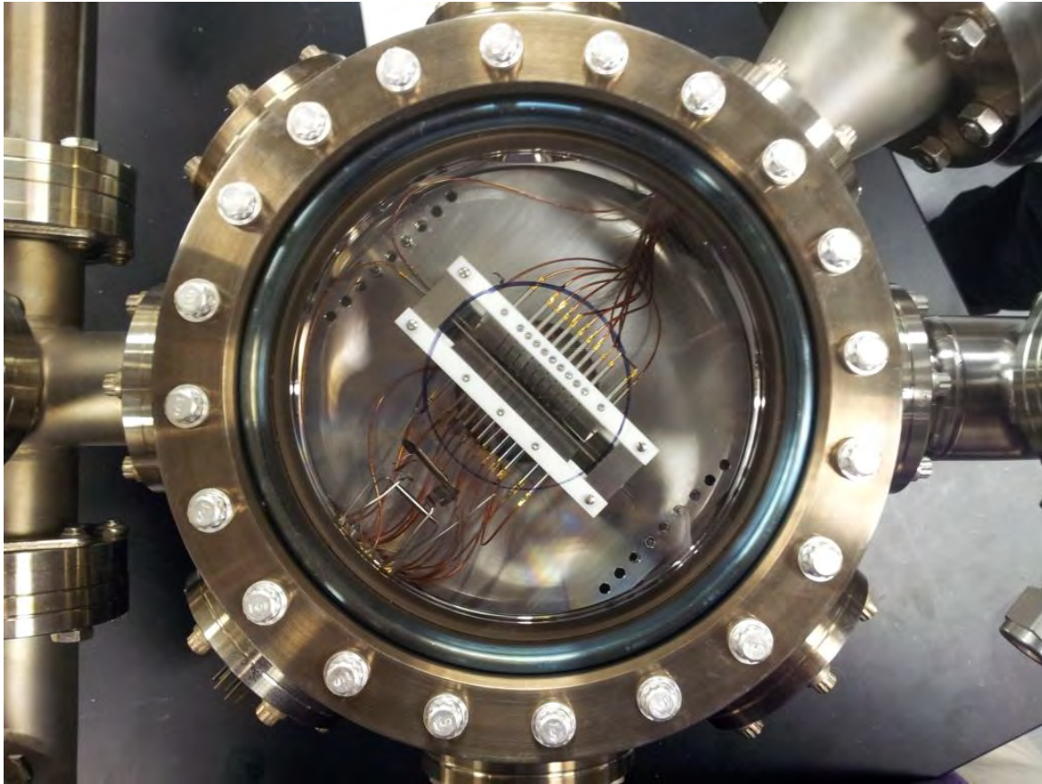
Figure 10: View of the Goeters trap within the vacuum chamber. The oven used for storage and sublimation of neutral calcium is visible just to the left of the ion trap..
