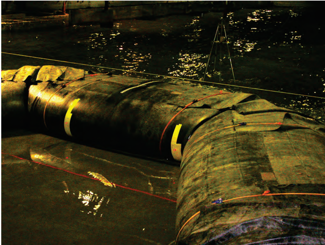
Figure 5-5. A Floodwall water-filled tube being tested in the laboratory in 2007.
