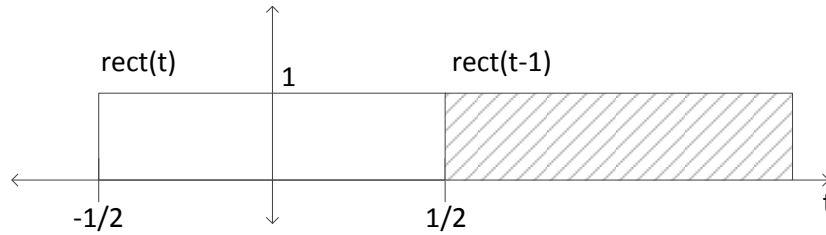
Figure 7. \text{rect}(t)\text{rect}(t - 1) .
