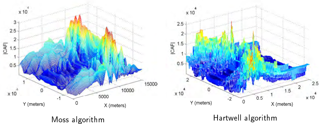
Figure 17. N = 2^{14} , dm = 100 , SNR = 10 dB, 30 Snapshots, Full Map.
