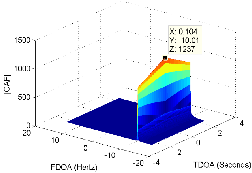
Figure 9. CAF of the example \text{rect}(t) signals, with offsets of 10 Hz in frequency, and 0.1 seconds in time.
