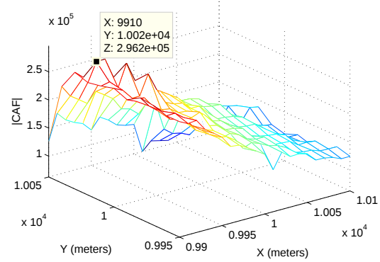
Hartwell algorithm
