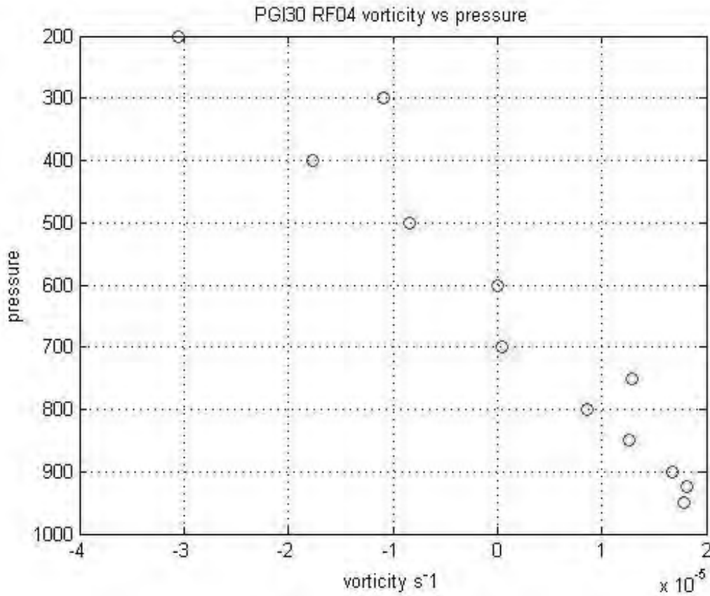
Figure 29. Vertical profile of area-averaged vorticity for Research Flight 04 (in PGI30) for the path shown in Figure 28. Vorticity is plotted in units of 10^{-5} \text{ s}^{-1} . Image derived from NSF GV dropsondes.
