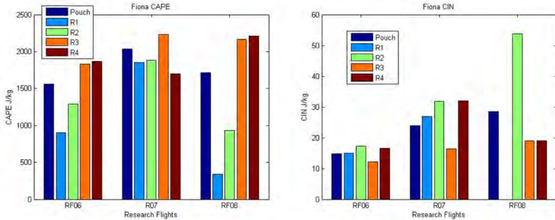
Figure 37. CAPE and CIN for RF06, RF07, and RF08 plotted according to the dropsondes distance from the sweet spot. Refer to Figure 13 for explanation of graphic. Images derived from NSF GV dropsondes.
