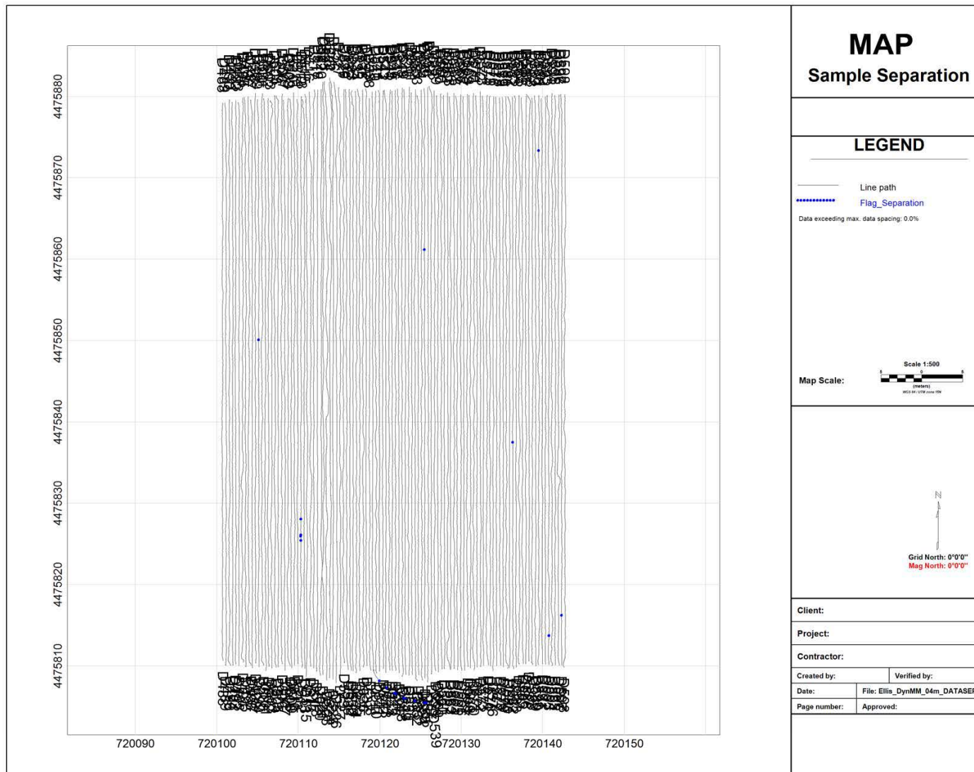
Figure 7-7: Partial MetalMapper Dataset Along-line Measurement Spacing
