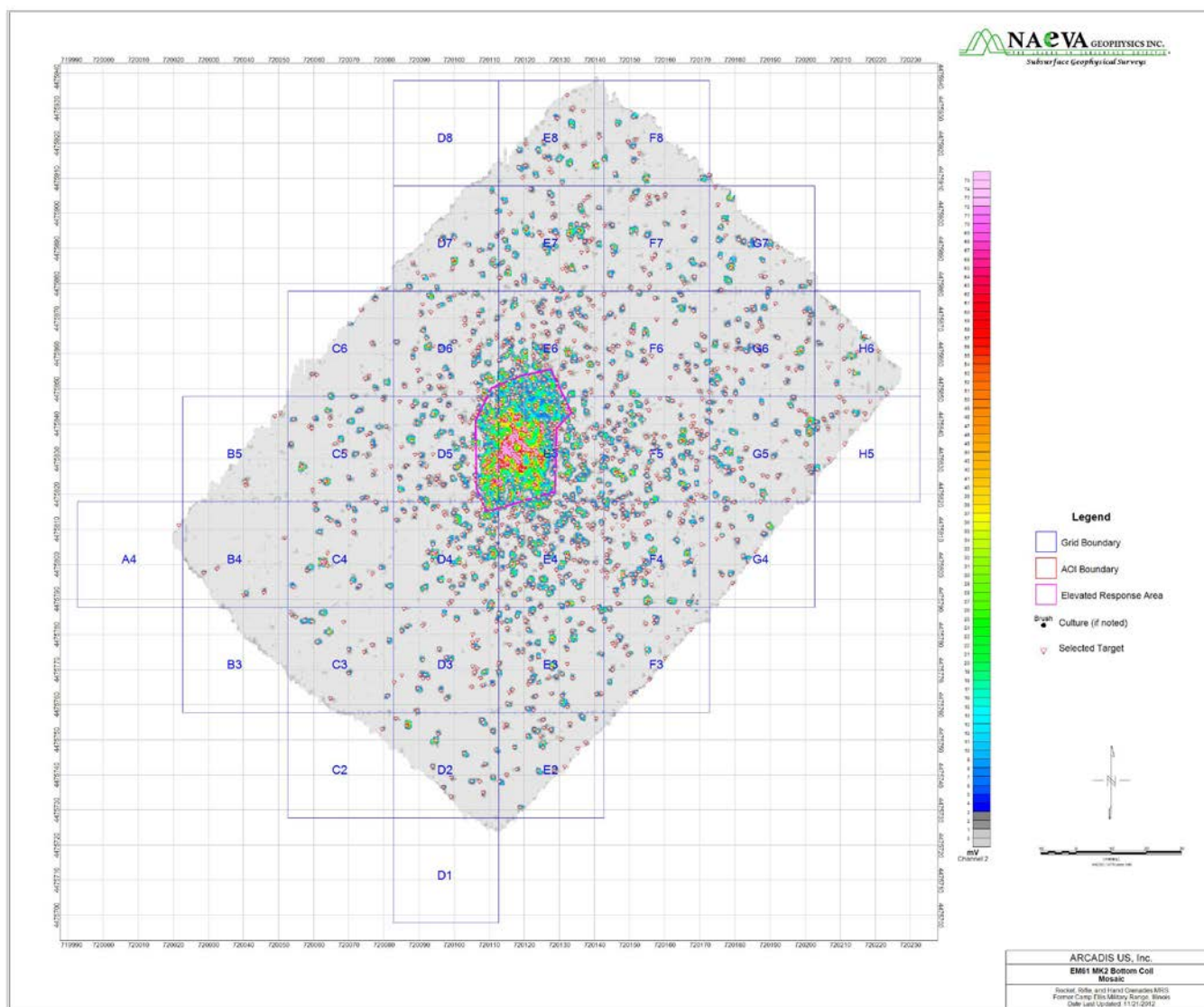
Figure 6-1: Dynamic EM61-MK2 Data
