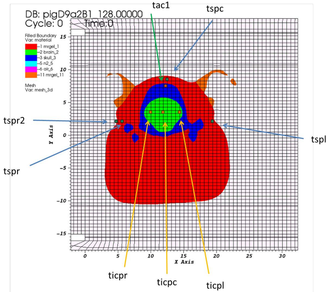
Fig. 5 Locations of the tracers in the coarser mesh ( Z = -2 plane)
