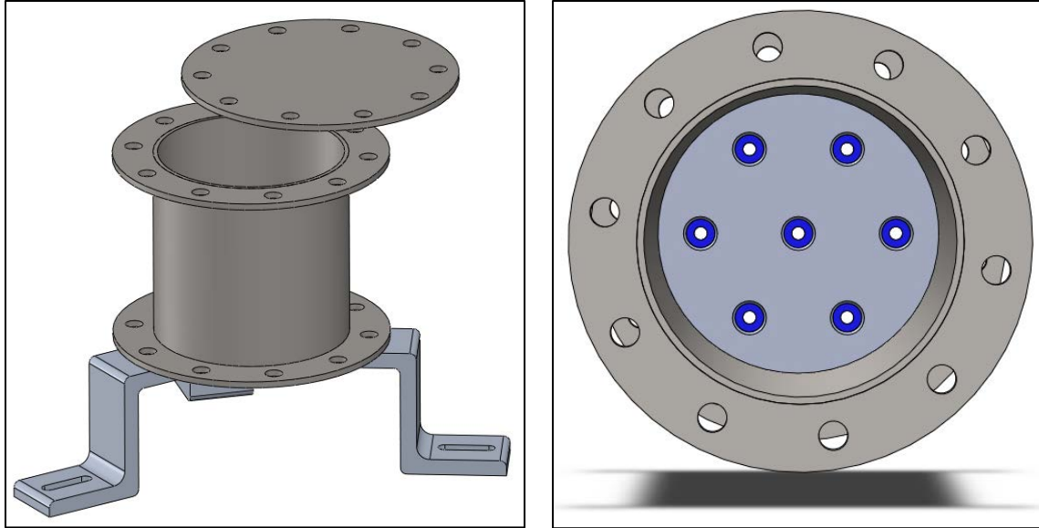
Figure 8. The UV reactor (left) is an adaptation of a design by Michael Spencer, AFIT [11]. The right picture displays the top view of the reactor which houses 7 silicon sealed LEDs (blue) that irradiate from the bottom. Composed of electropolished stainless steel, the reactor allows for a high reflectance. The lid swivels, as shown on the left, for facilitated sample collection. The reactor rested upon three standoffs that are attached to a shaker. The shaker helped to prevent spores from clumping or aggregating to the sides of the reactor. Models were created using SolidWorks software.
