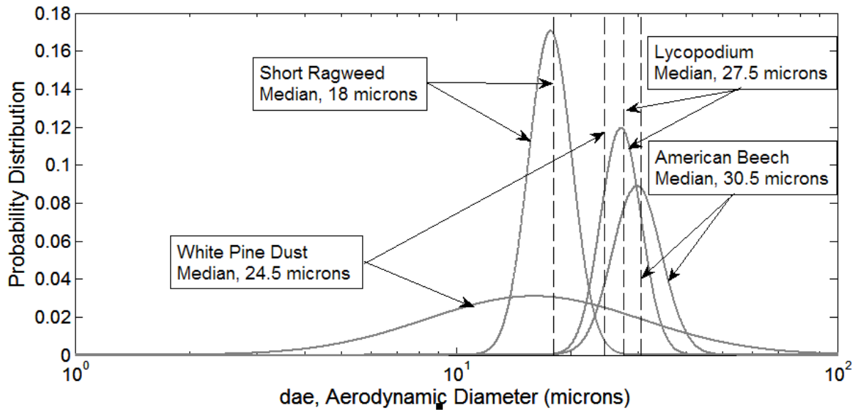
Figure 3. Particle size distributions of the Breyse and Swift particles.
