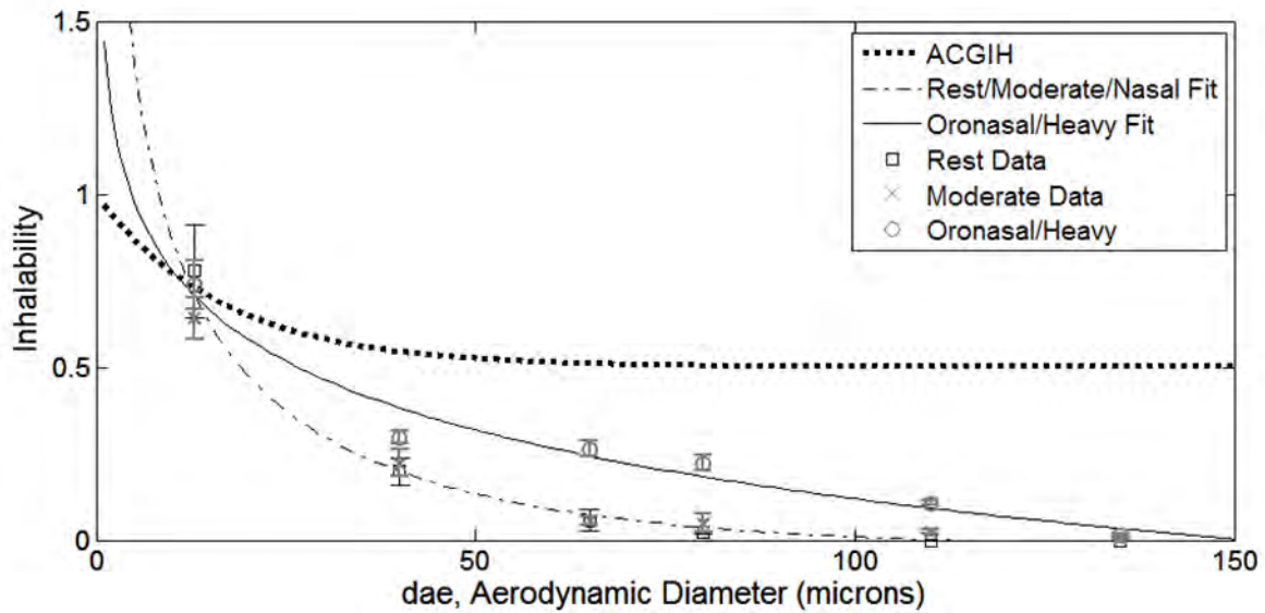
Figure 7. Hsu's data and his original quadratic polynomial curve-fits.
