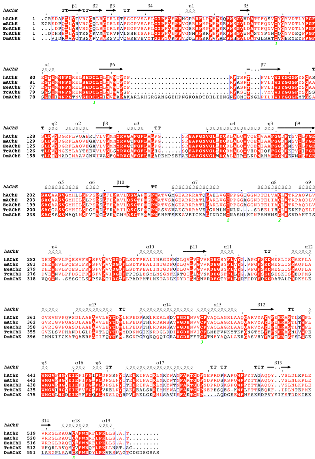
Fig. 8. Sequence alignment of AChEs whose 3D structures have been solved
