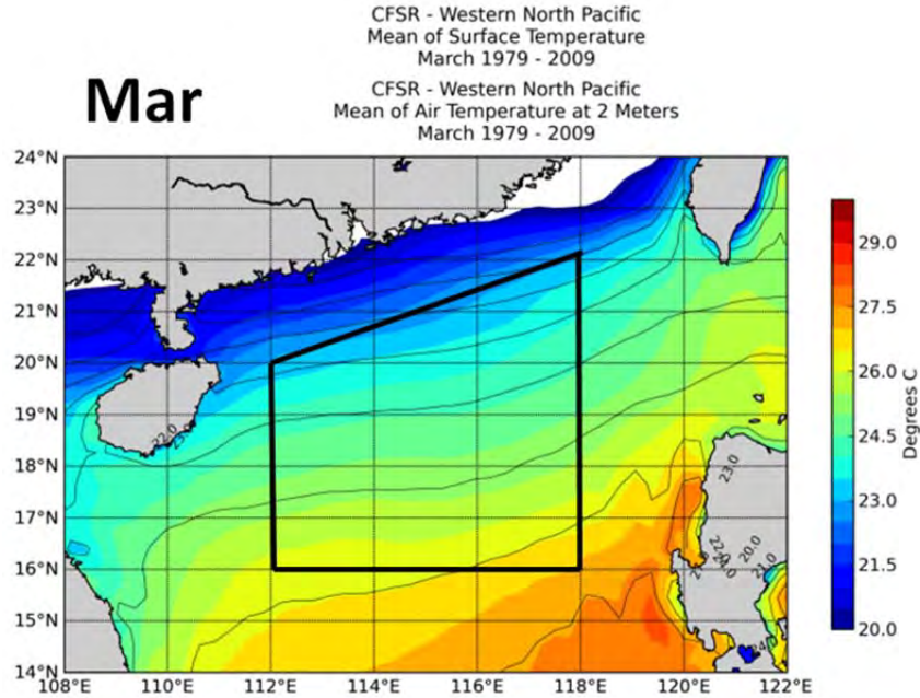
Figure 23. LTM SST (color fill) and 2 m AT (black contours). Area-averaged LTM: AT = 24.3^{\circ}\text{C} , SST = 24.8^{\circ}\text{C} , ASTD = -0.48^{\circ}\text{C} . Area averaged monthly mean ranges: AT: 23.1^{\circ} to 25.7^{\circ} , SST: 23.8^{\circ} to 26.1^{\circ} , ASTD: -0.99^{\circ} to -0.14^{\circ} . Figure created at the ACAF website (October 2013).
