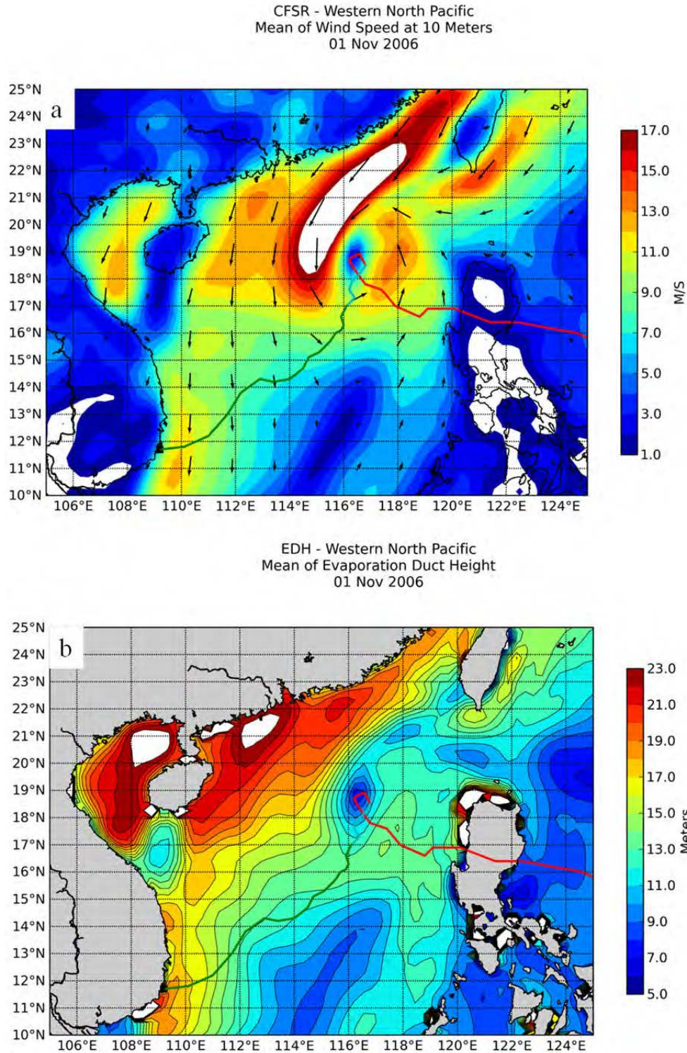
Figure 48. Impacts on SCS EDH of a tropical cyclone in the SCS on November 1, 2006. Figure 48a depicts the daily mean wind field and Figure 48b depicts the daily mean EDH. The red and green line shows the track of this TC. Figures created at the ACAF website (October 2013).
