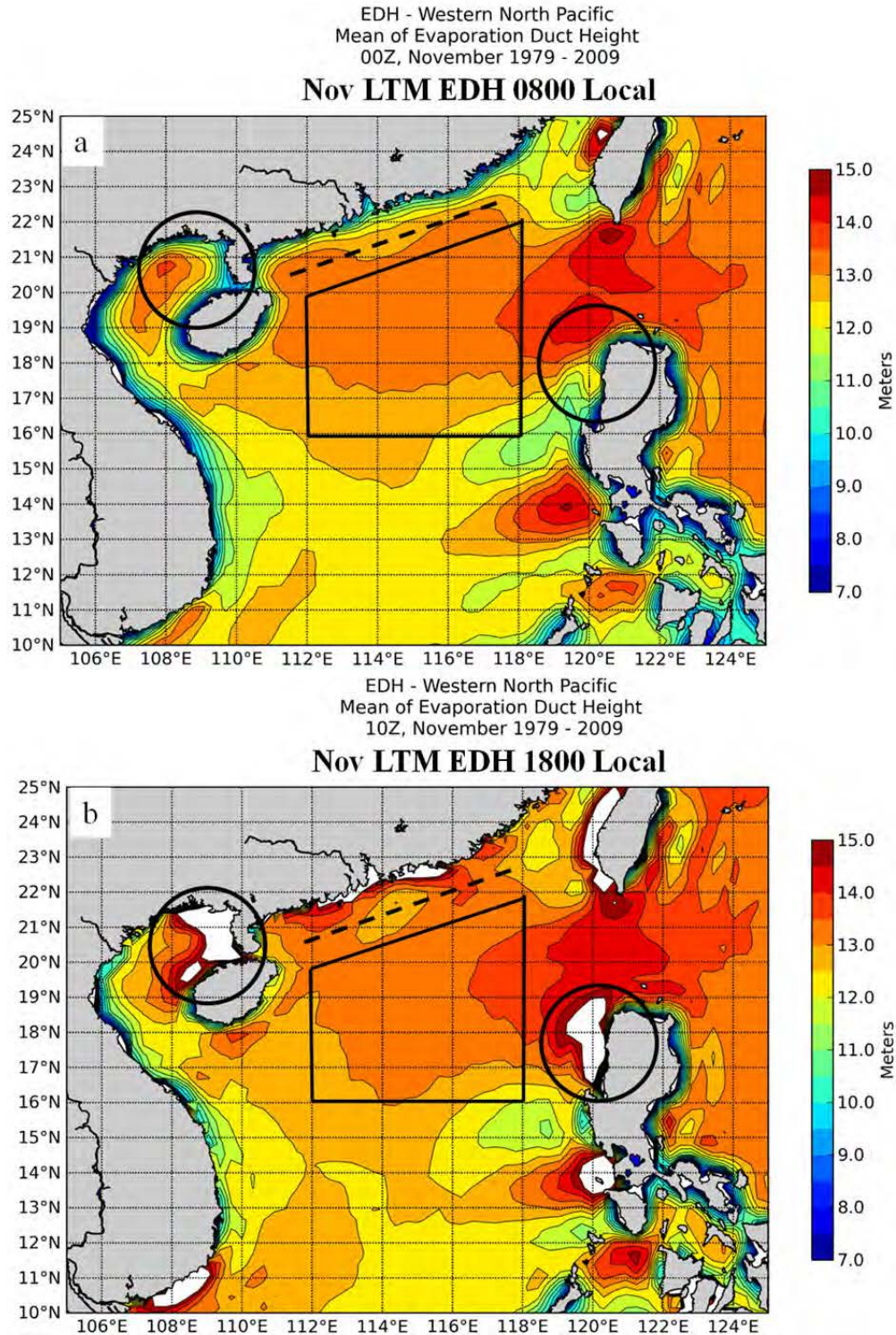
Figure 46. Diurnal and coastal variations in November LTM EDH. EDH at (a) 0800 local and (b) 1800 local show regions of significant coastal and diurnal variation (circled areas). The dashed line identifies a coastal region discussed in the main text. Figures created at the ACAF website (October 2013).
