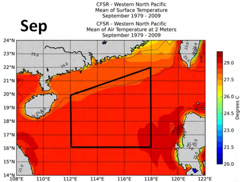
Figure 25. LTM SST (color fill) and 2 m AT (black contours). Area-averaged LTM: AT = 28.3^{\circ}\text{C} , SST = 28.7^{\circ}\text{C} , ASTD = -0.45^{\circ}\text{C} . Area averaged monthly mean ranges: AT: 27.5^{\circ} to 29.1^{\circ} , SST: 27.6^{\circ} to 29.8^{\circ} , ASTD: -0.99^{\circ} to 0.05^{\circ} .
