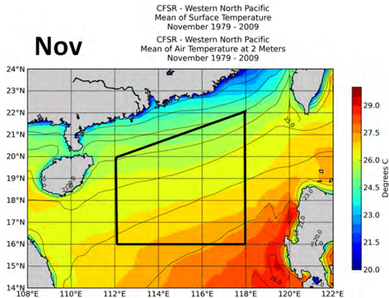
Figure 26. LTM SST (color fill) and 2 m AT (black contours). Area-averaged LTM: AT = 25.4^{\circ}\text{C} , SST = 26.3^{\circ}\text{C} , ASTD = -0.93^{\circ}\text{C} . Area averaged monthly mean ranges: AT: 24.1^{\circ} to 26.5^{\circ} , SST: 25.1^{\circ} to 27.4^{\circ} , ASTD: -1.36^{\circ} to -0.25^{\circ} .
