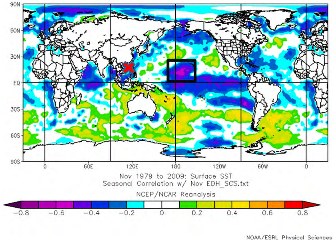
Figure 45. Plot of correlation between SCS EDH and SST in November. The global maximum correlation values are +0.55 and -0.71. The red X indicates the northern SCS study region. Figure created at the ESRL website (October 2013).
