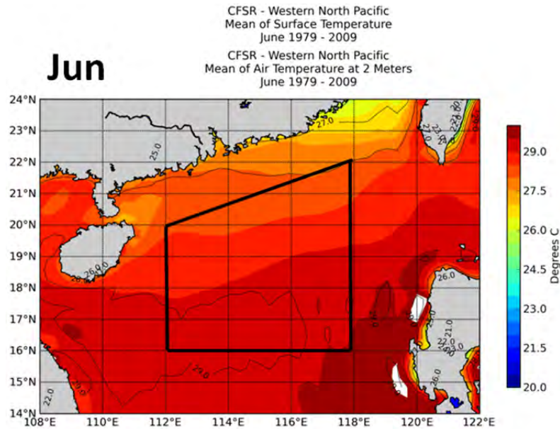
Figure 24. LTM SST (color fill) and 2 m AT (black contours). Area-averaged LTM: AT = 28.8^{\circ}\text{C} , SST = 28.9^{\circ}\text{C} , ASTD = -0.12^{\circ}\text{C} . Area averaged monthly mean ranges: AT: 28.2^{\circ} to 29.6^{\circ} , SST: 28.1^{\circ} to 29.7^{\circ} , ASTD: -0.44^{\circ} to 0.16^{\circ} . Figure created at the ACAF website (October 2013).
