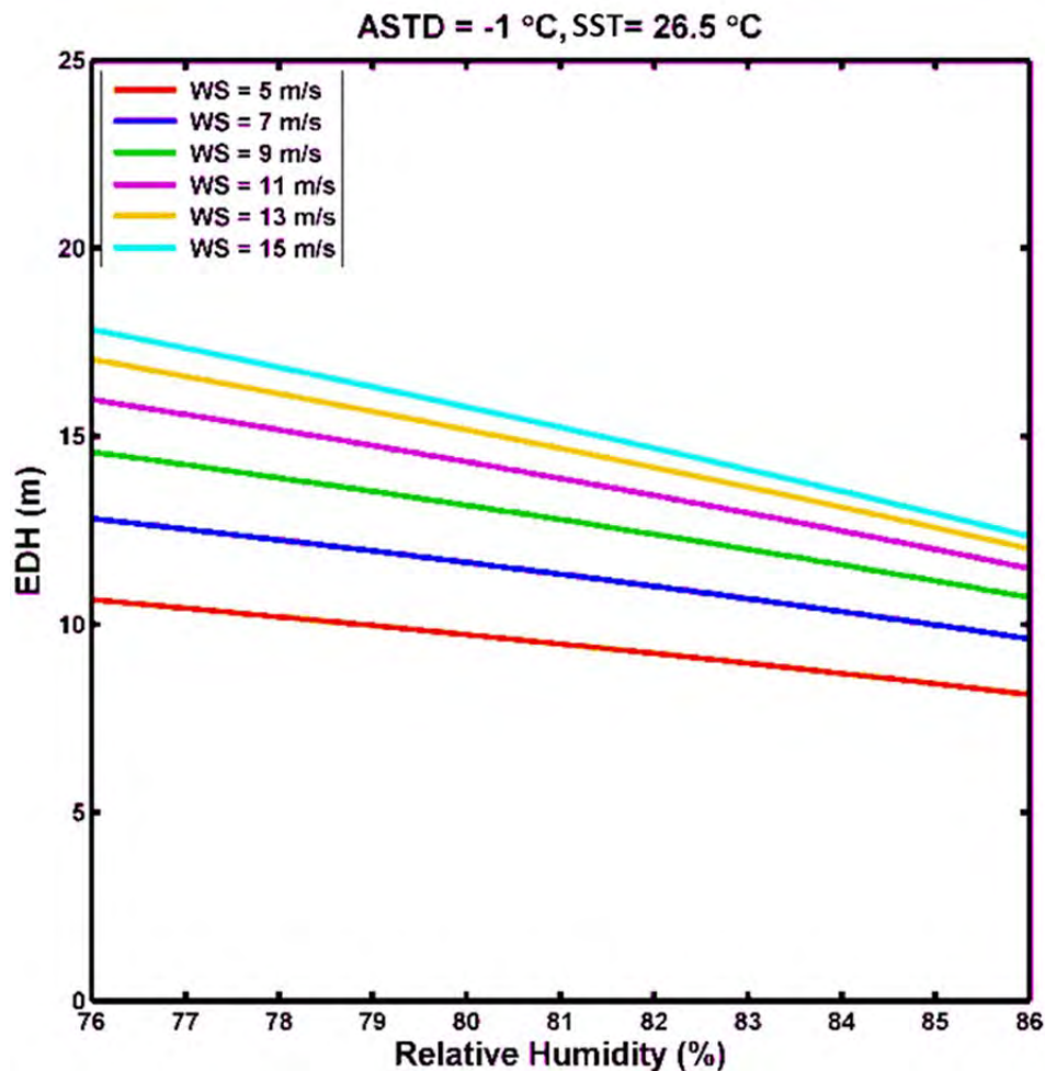
Figure 27. EDH versus RH for various wind speeds. Note the increased negative slope for higher winds speeds. Plot of NAVSLaM-modeled EDH courtesy of Paul Frederickson (October 2013).
