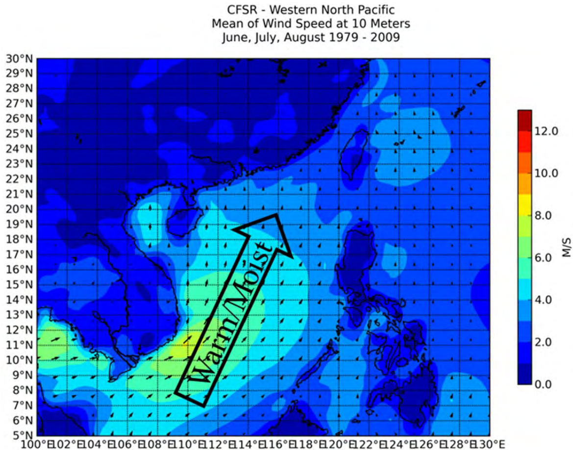
Figure 19. June-August mean near-surface wind speed and direction. Moderate SW winds into the SCS from the maritime continent bring warm, moist air into the SCS. This causes a local maximum in evaporation duct heights. Figure created at the ACAF website (October 2013).
