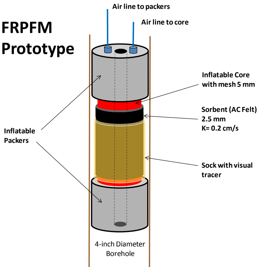
Figure 24. FRPFM Laboratory-Scale Prototype (Insert shows laboratory-scale prototype).
