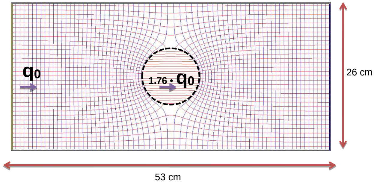
Figure 28. Simulated flow streamlines from the fracture flow simulator under open borehole conditions.
