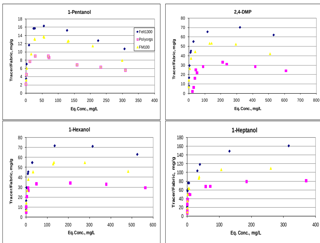
Figure 16. Adsorption isotherm of resident alcohol tracers on AC Felt1300, FM 100 cloth, and Polyorgs.
