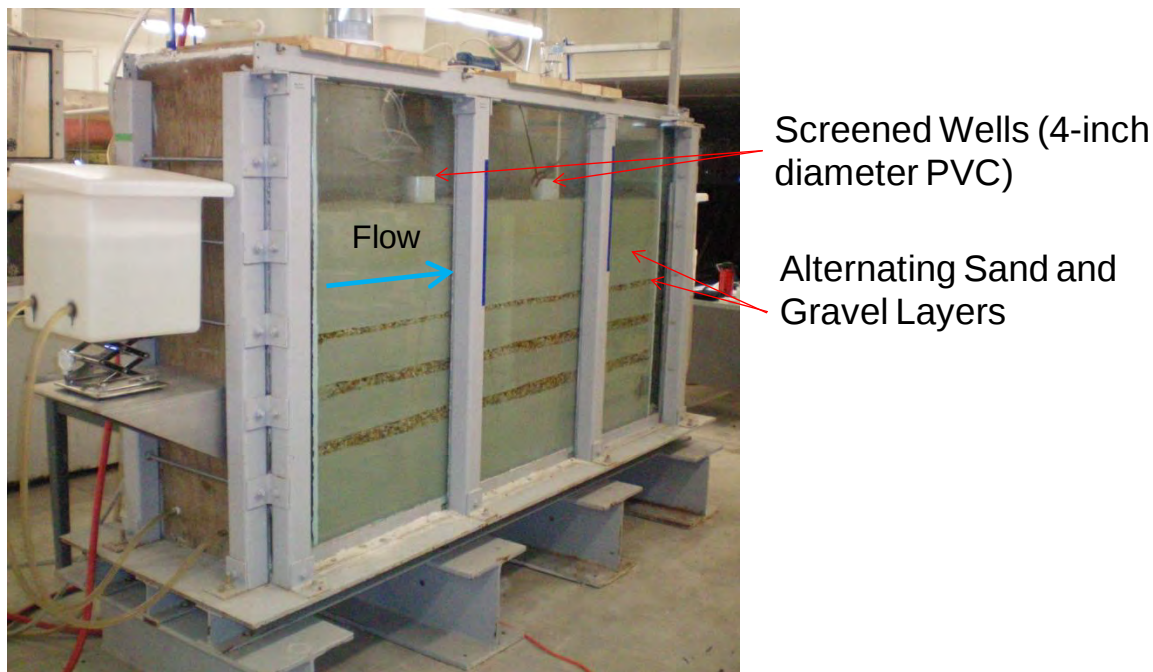
Figure 22. Aquifer box: screened-well high contrast flow simulator.
