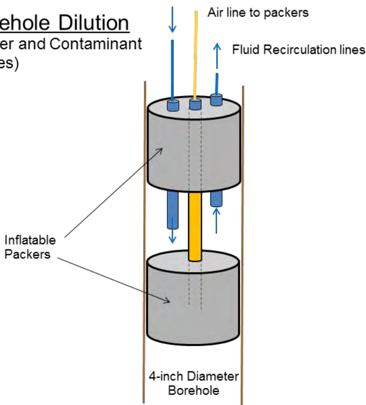
Figure 25. Schematic and image of laboratory-scale borehole dilution apparatus.
