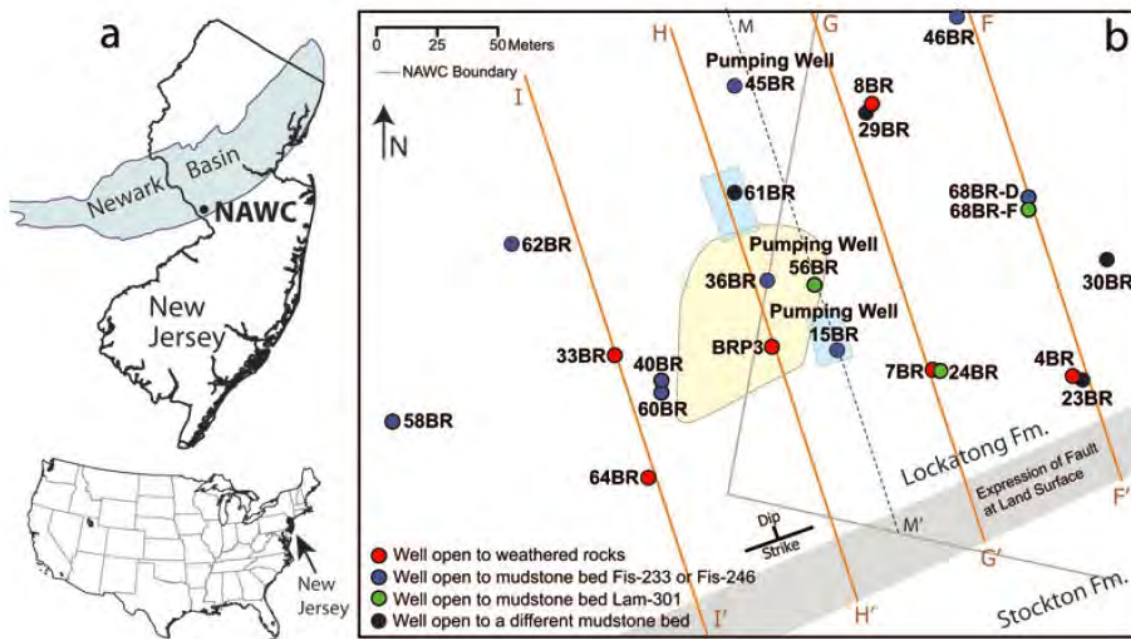
Figure 13. (a) Location of the former Naval Air Warfare Center (NAWC) site in West Trenton, NJ. (b) Plan view of NAWC site showing locations of pumping and monitoring wells. (Tiedeman et al, 2010).
