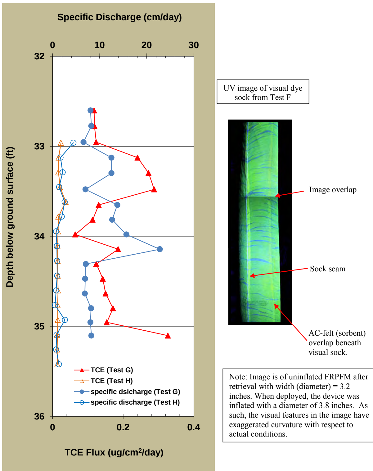
Figure 42. Summary of flux measurements and visual results for Tests F, G, and H comparing vertical distribution of water flux (specific discharge), contaminant flux and presence of flowing fractures.
