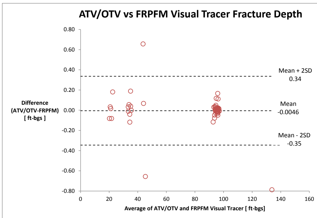
Figure 58. Summary of statistical analysis for data type 2A—fracture location by ATV/OTV and FRPFM visual tracers.
