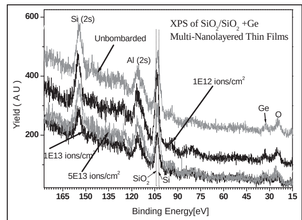
Figure 2. XPS spectra of \text{SiO}_2/\text{SiO}_2 + \text{Ge} multinanolayered thin films at different fluences. XPS: X-ray photoelectron spectroscopy.
