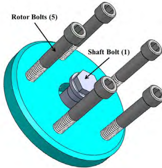
Figure 36. Attachment bolts
