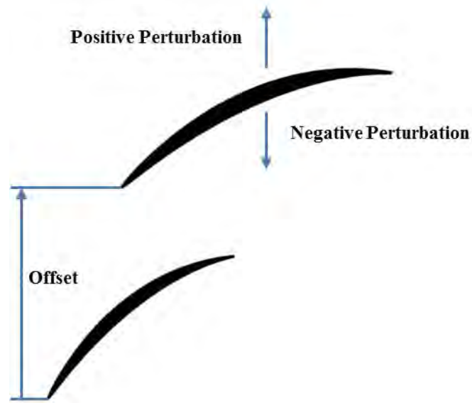
Figure 31. Offset perturbation
