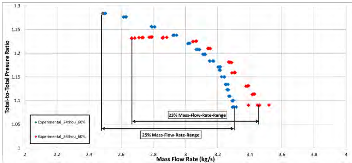
Figure 25. Experimental pressure ratio versus mass flow for decreasing tip gap (after [1])
