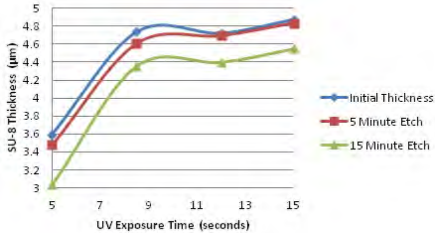
Figure 76. Plot of the average SU-8 thicknesses with respect to UV exposure time for the initial thickness, following a 5 minute plasma etch, and following a 15 minute plasma etch.
