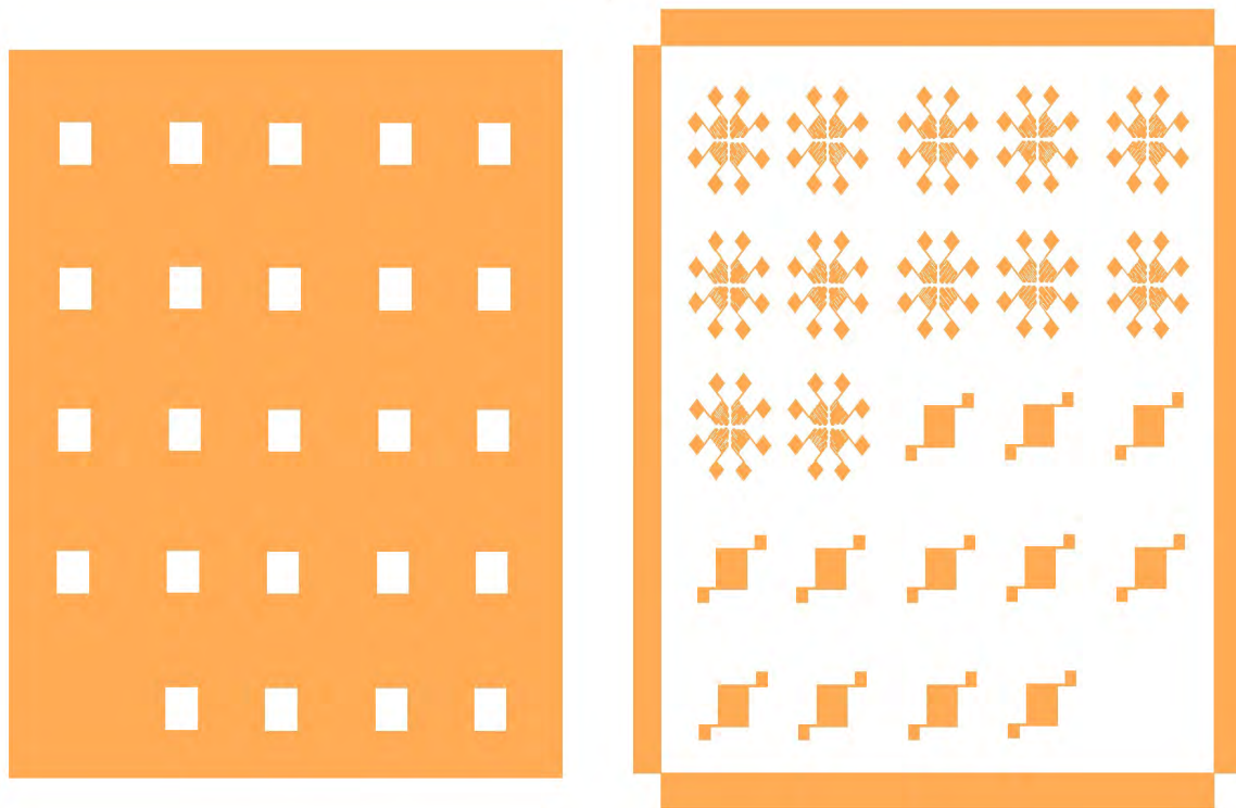
Figure B-3. Mask pattern for fabrication of multidirectional heaters and membranes.
