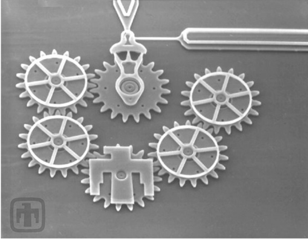
Figure 6. Scanning electron microscope (SEM) image of a MEMS gear chain fabricated using the SUMMiT V process [13].
