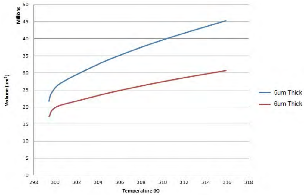
Figure 72. Plot of the membrane volume vs. temperature for a 1.0\text{mm} \times 1.0\text{mm} membrane.
