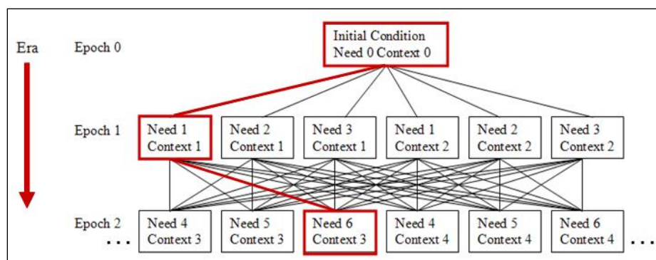
Figure 8. Eras generated as path through possible epoch space (from Ross et al. 2008 61 )
