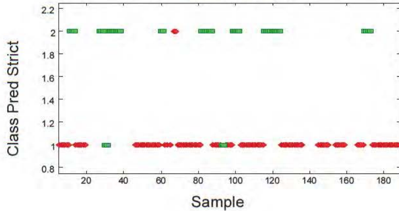
Cross-validation Data
