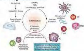
Fig 1 Ischemia-Reperfusion Injury
