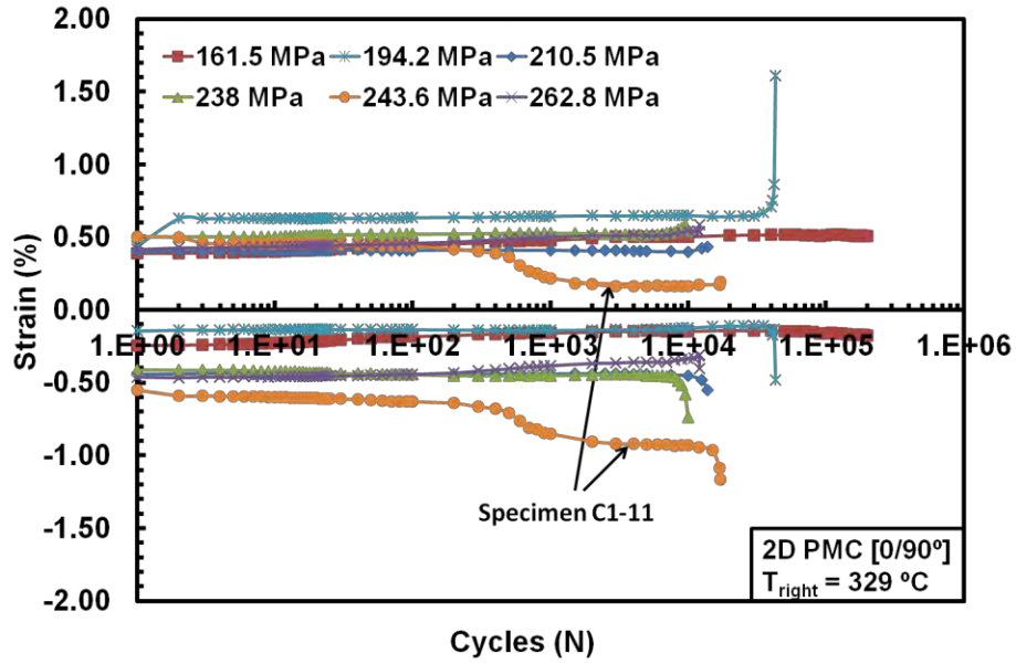
Figure 42: Maximum and minimum strain vs. tension-compression fatigue cycles for the 2D PMC with 0/90° fiber orientation at elevated temperature.
