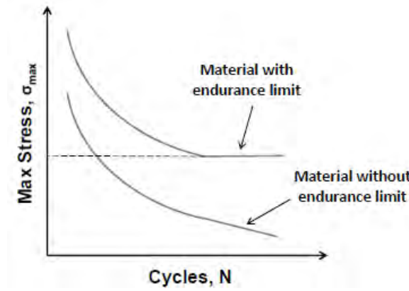
Figure 5: Example of S-N curve.
