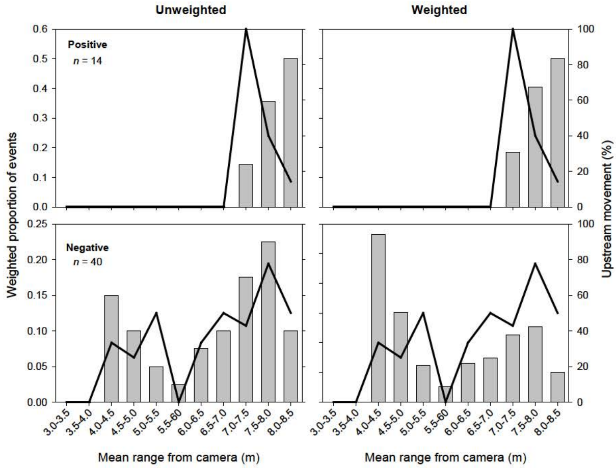
Figure 28. Observed (unweighted) and weighted proportions of events observed in relation to mean distance from camera at JD3 cross section during landscape tilting DIDSON deployment. Solid line shows the percentage of events in each bin that were moving upstream. The weighting adjusted for smaller observed volume closer to the camera.
