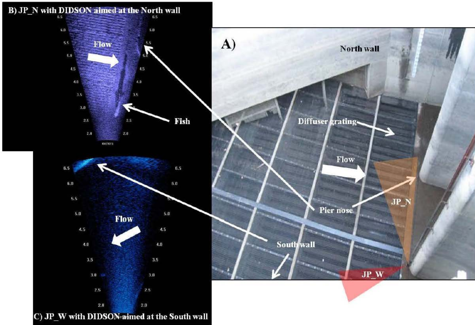
Figure B2. A) DIDSON camera deployments at the Junction Pool of Bonneville Dam with B) JP North landscape view and C) JP West landscape view.
