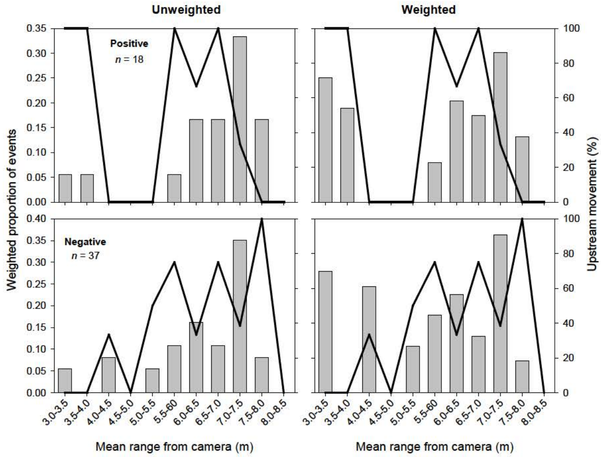
Figure 29. Observed (unweighted) and weighted proportions of events observed in relation to mean distance from camera at JD3 turnpool (TP) during landscape tilting DIDSON deployment. Solid line shows the percentage of events in each bin that were moving upstream. The weighting adjusted for smaller observed volume closer to the camera.
