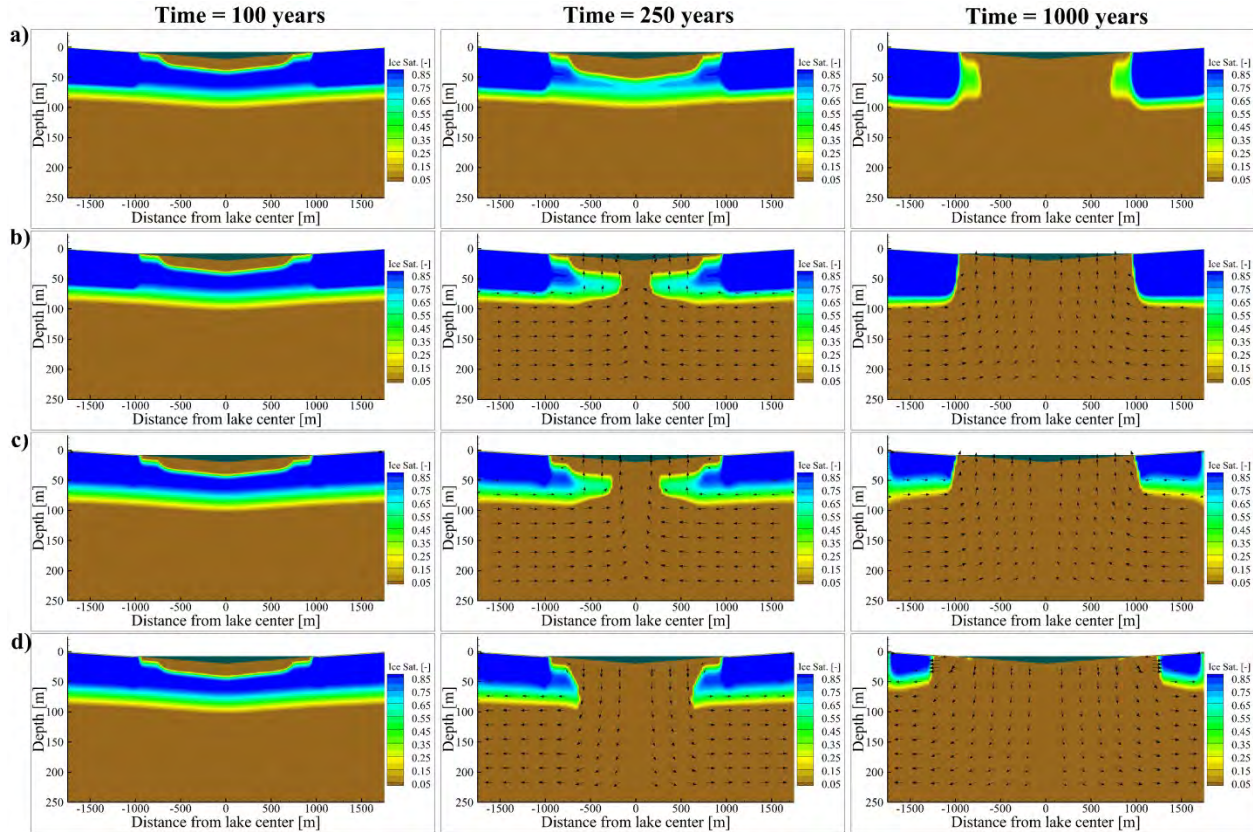
Figure 5.4.2.2 Cross-sections of 2D cylindrical model (mirrored) showing states of lake- talik formation, ice saturation, and groundwater movement where a 12m lake forms over a continuous permafrost layer of about 90m in thickness.
