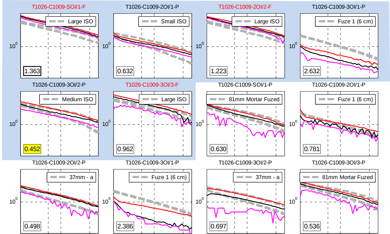
Figure 3. Polarizabilities for missed QC seed WK-707 (37mm APT at 20 cm depth). The first six models (light blue background) used data background corrected using the nearest in-air measurement and, for the two-object (2OI) and three-object (3OI) inversions, fixing one of the sources at 90 cm depth. The remaining six models used data that were corrected using the nearest near-ground background correction. Red, black and magenta lines are predicted polarizabilities. Broken grey lines are best fitting reference library polarizabilities. The predicted polarizabilities for all models are typical of a soil response. None of the models remotely resemble any of the 37mm reference items.
