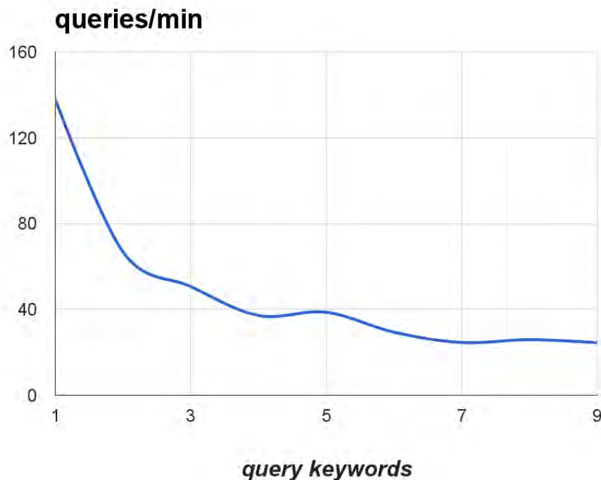
Figure 14. End-to-end performance of a single SCPU-based boolean keyword search query interface on a 1TB database with 4KB blocks and a small dictionary of 1600 keywords in a constrained remote client network setup (3ms latencies, 10Mbps bandwidth). Throughput decreases with increasing number of query keywords.
