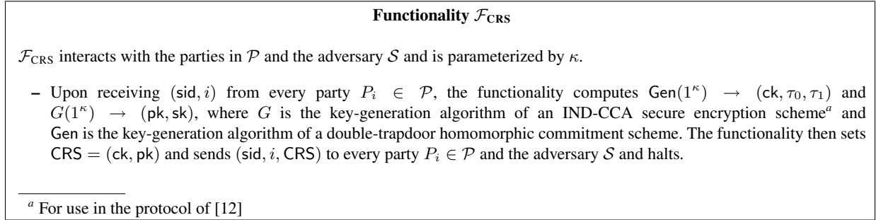
Fig. 2. The Ideal Functionality for Generating CRS
