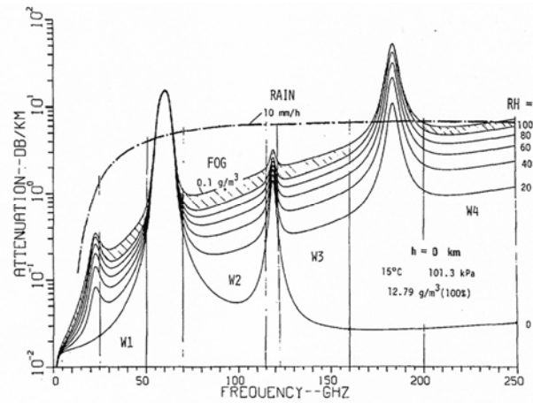
Fig. 1.19: Atmospheric attenuation at sea level for various relative humidity levels [10].
