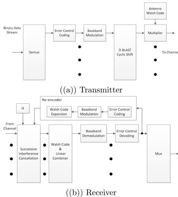
Figure 13: Variable rate MIMO transceiver block diagram
