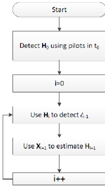
Figure 8: Scheme 1 Flowchart. l_i = [\mathbf{s}_{1,i} \mathbf{s}_{2,i+1} \dots \mathbf{s}_{t,i+t-1}] , \mathbf{H}_i = [\mathbf{h}_1^{(i)} \mathbf{h}_2^{(i)} \dots \mathbf{h}_t^{(i)}]
