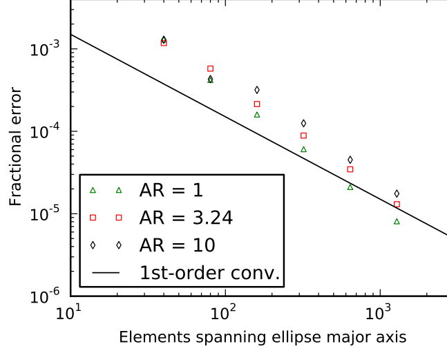
Fig. 11: Results of spatial mesh refinement convergence study for elliptical inclusions with various aspect ratios, showing fractional error relative to the respective exact solution as a function of N , for regular-mesh simulations.
