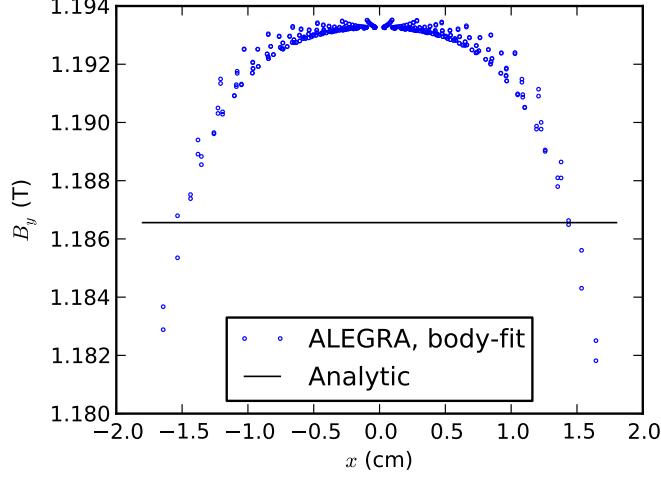
Fig. 6: Spatial distribution of deviation from exact solution for B_2 at equilibrium for body-fitted mesh with N = 40 .
