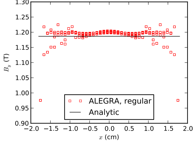
Fig. 7: Spatial distribution of deviation from exact solution for B_2 at equilibrium for regular mesh with N = 40 .
