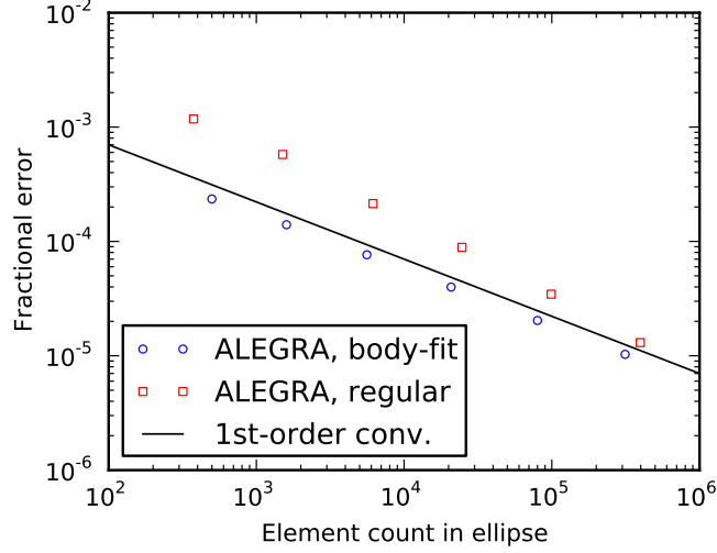
Fig. 9: Results of spatial mesh refinement convergence study for an elliptical inclusion, showing fractional error relative to exact solution.
