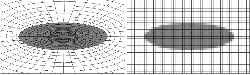
Fig. 2: Zoomed-in view of meshes used for ALEGRA simulations: body-fitted (left) and regular (right).
