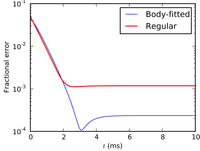
Fig. 8: Time evolution of RMS deviation of ALEGRA solution relative to exact solution for equilibrium condition at N = 40 .
