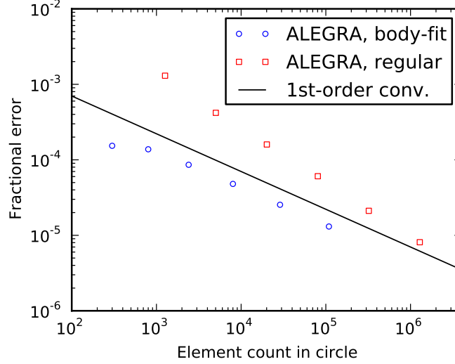
Fig. 10: Results of spatial mesh refinement convergence study for a circular inclusion, showing fractional error relative to exact solution.
