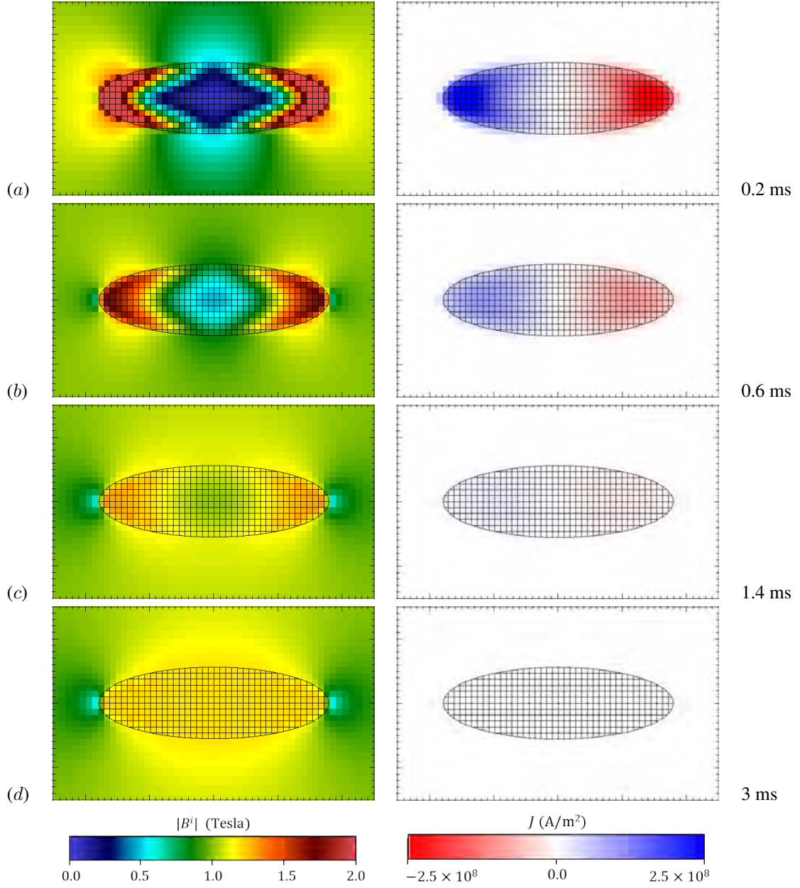
Fig. 5: Simulation evolution for regular mesh: B^i magnitude (left) and J magnitude (right), with mesh lines in the ellipse superimposed. Simulation times: a) 0.2 ms, b) 0.6 ms, c) 1.4 ms, d) 3 ms. Blue-red colorbar for B^i spans 0 \leq |B^i| \leq 2 T.
