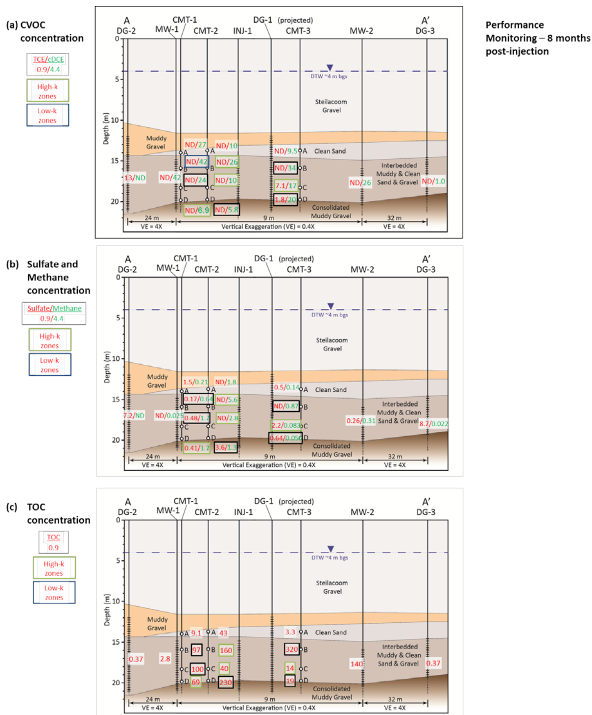
Figure 5.28. Groundwater sampling results from performance monitoring – 8 months post injection. The location of cross-section A-A' is shown in Figure 5.2.
