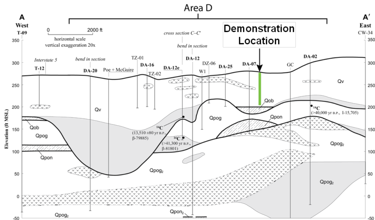
Figure 4.4. Conceptual geologic cross-section A-A' (see Figure 4.3 for transect location). The cross section (adapted from Borden and Troost, 2001) is generally located along the centerline of the Area D plume in the Vashon Aquifer. For the cross section, white areas (Qv, Qpog, Qpog 2 ) correspond to outwash gravels, the grey area is glaciolacustrine aquitard sediment, Qob is Olympia bed material, the hashed areas (Qpon and Qpon 2 ) are non-glacial aquitard materials, and the areas with the “v” symbol pattern correspond to till material. The Vashon Aquifer lies above the uppermost Qpon aquitard.
